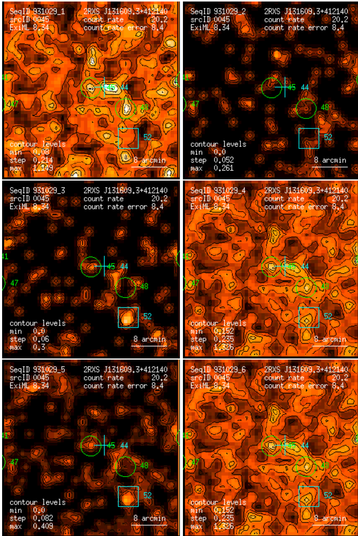
Figure 45: RASS 931029: detection 0045: band rate images, Gaussian filter: (1) PSPC channels 11 – 41, (2) 52 – 90, (3) 91 – 201, (4) 11 – 235, (5) 52 – 201, (6) 11 – 201. Broad band rates in counts/ks. Band rate contour levels in counts/ks/arcmin 2 .
