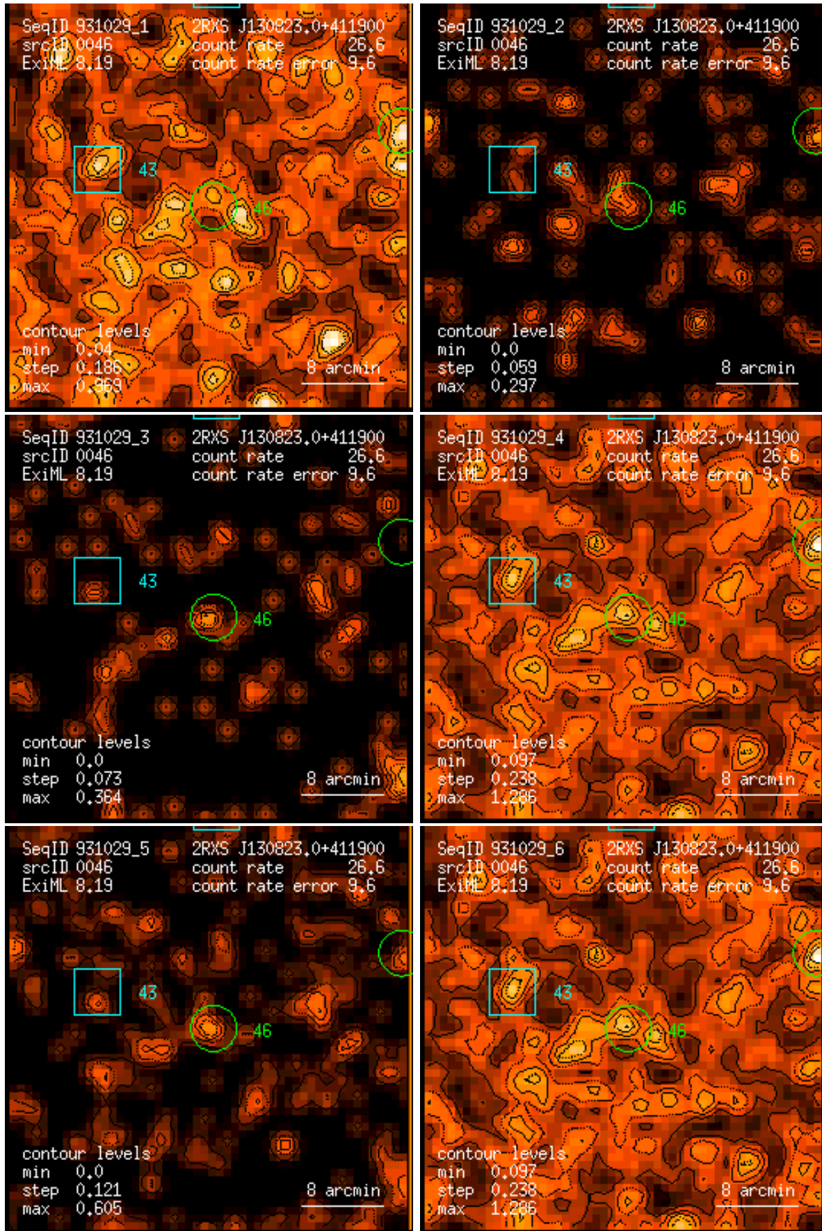
Figure 46: RASS 931029: detection 0046: band rate images, Gaussian filter: (1) PSPC channels 11 – 41, (2) 52 – 90, (3) 91 – 201, (4) 11 – 235, (5) 52 – 201, (6) 11 – 201. Broad band rates in counts/ks. Band rate contour levels in counts/ks/arcmin 2 .
