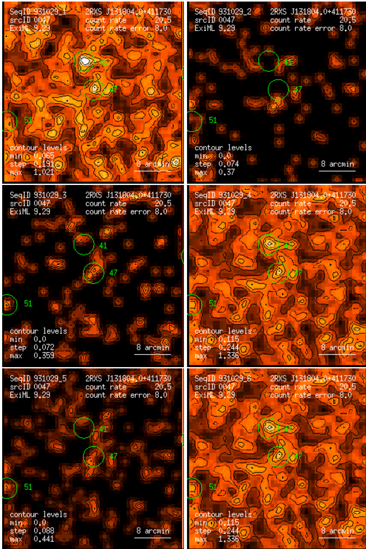
Figure 47: RASS 931029: detection 0047: band rate images, Gaussian filter: (1) PSPC channels 11 – 41, (2) 52 – 90, (3) 91 – 201, (4) 11 – 235, (5) 52 – 201, (6) 11 – 201. Broad band rates in counts/ks. Band rate contour levels in counts/ks/arcmin 2 .
