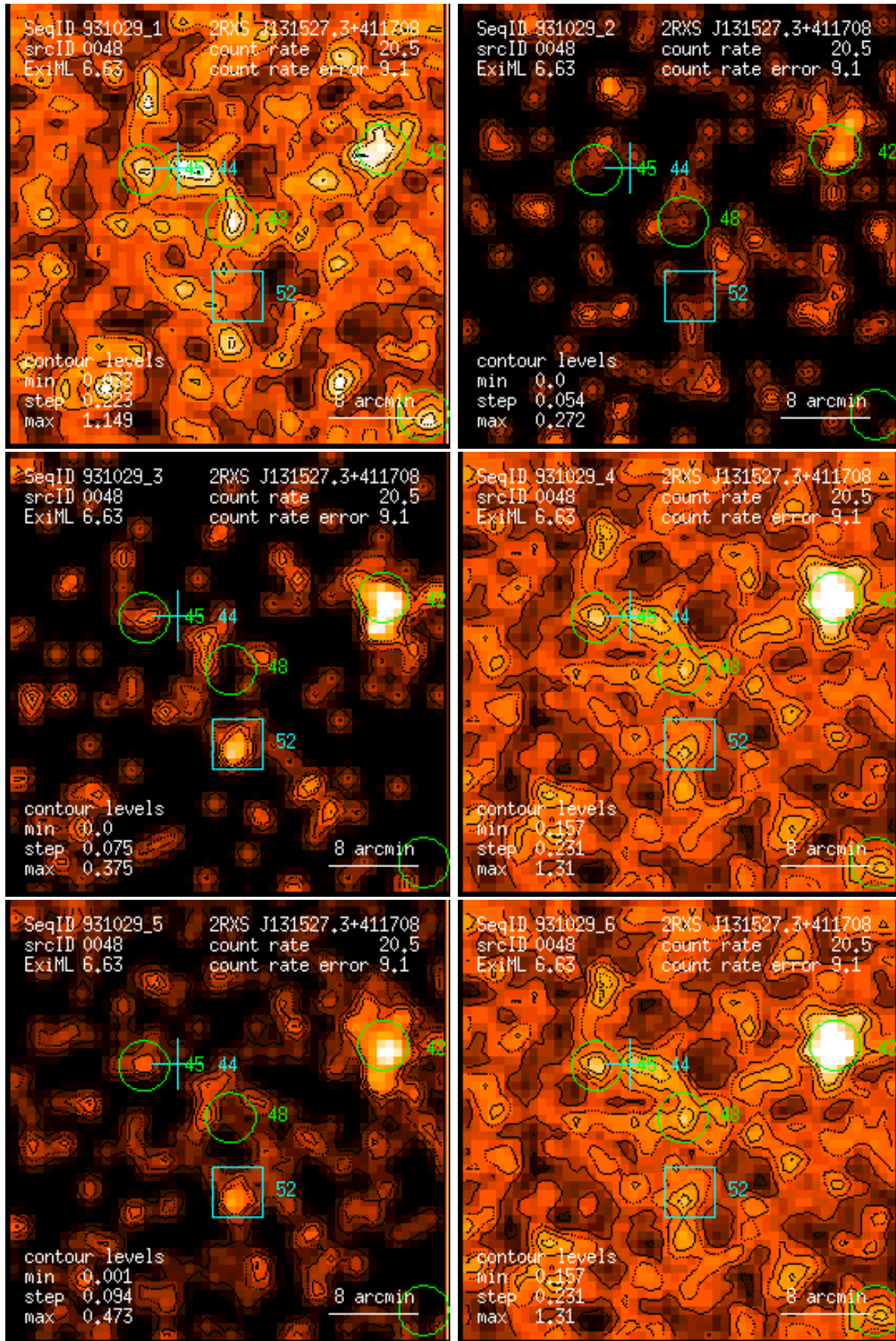
Figure 48: RASS 931029: detection 0048: band rate images, Gaussian filter: (1) PSPC channels 11 – 41, (2) 52 – 90, (3) 91 – 201, (4) 11 – 235, (5) 52 – 201, (6) 11 – 201. Broad band rates in counts/ks. Band rate contour levels in counts/ks/arcmin 2 .
