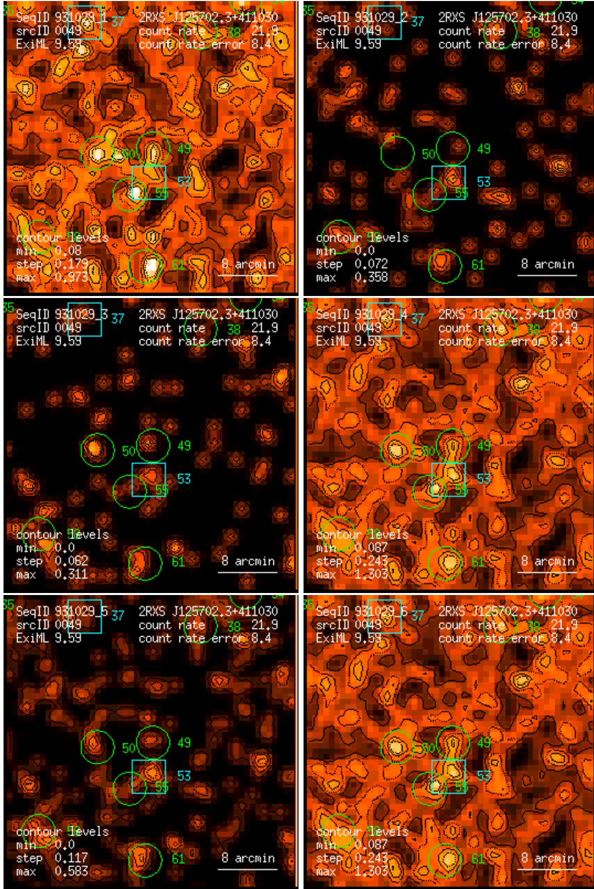
Figure 49: RASS 931029: detection 0049: band rate images, Gaussian filter: (1) PSPC channels 11 – 41, (2) 52 – 90, (3) 91 – 201, (4) 11 – 235, (5) 52 – 201, (6) 11 – 201. Broad band rates in counts/ks. Band rate contour levels in counts/ks/arcmin 2 .
