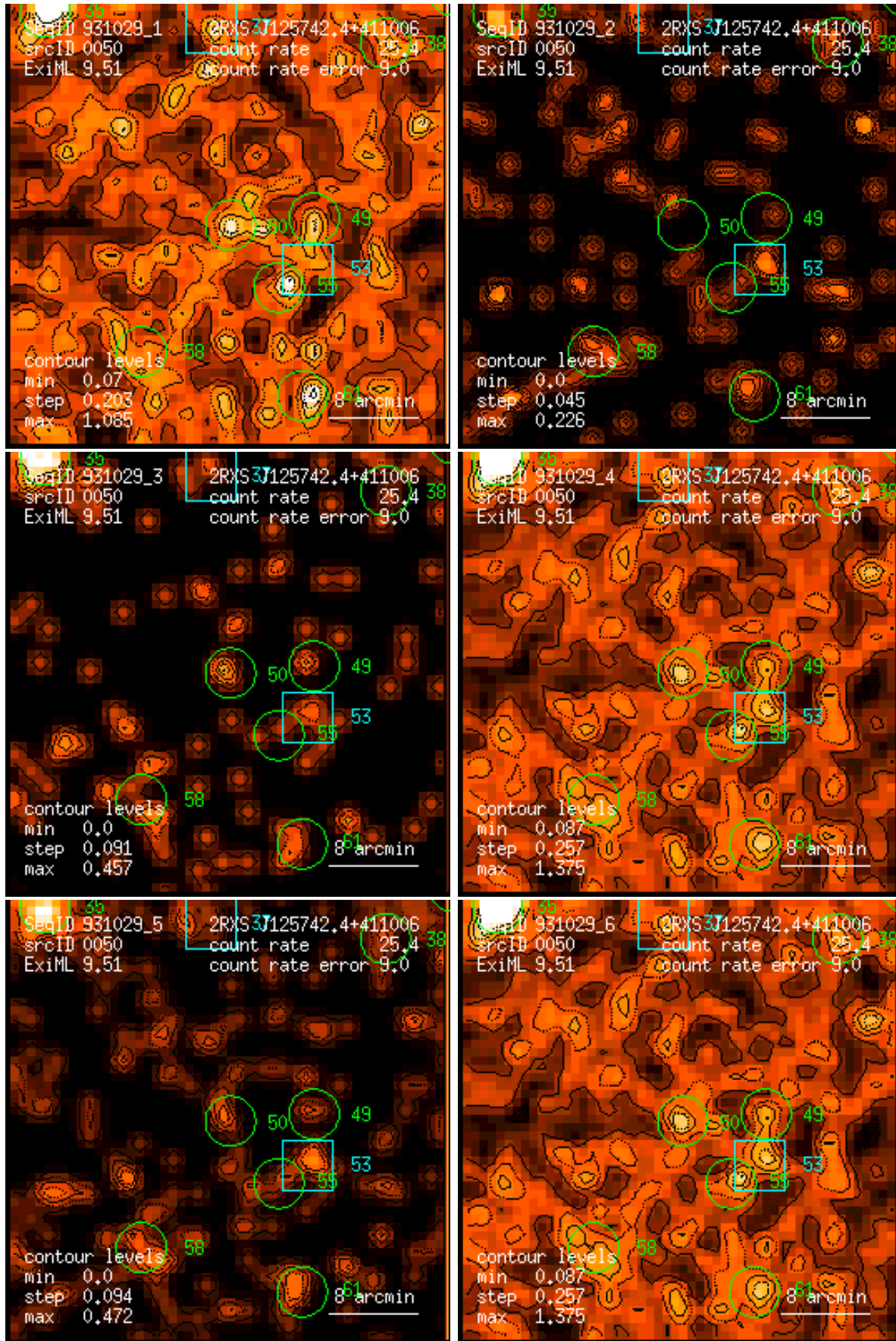
Figure 50: RASS 931029: detection 0050: band rate images, Gaussian filter: (1) PSPC channels 11 – 41, (2) 52 – 90, (3) 91 – 201, (4) 11 – 235, (5) 52 – 201, (6) 11 – 201. Broad band rates in counts/ks. Band rate contour levels in counts/ks/arcmin 2 .
