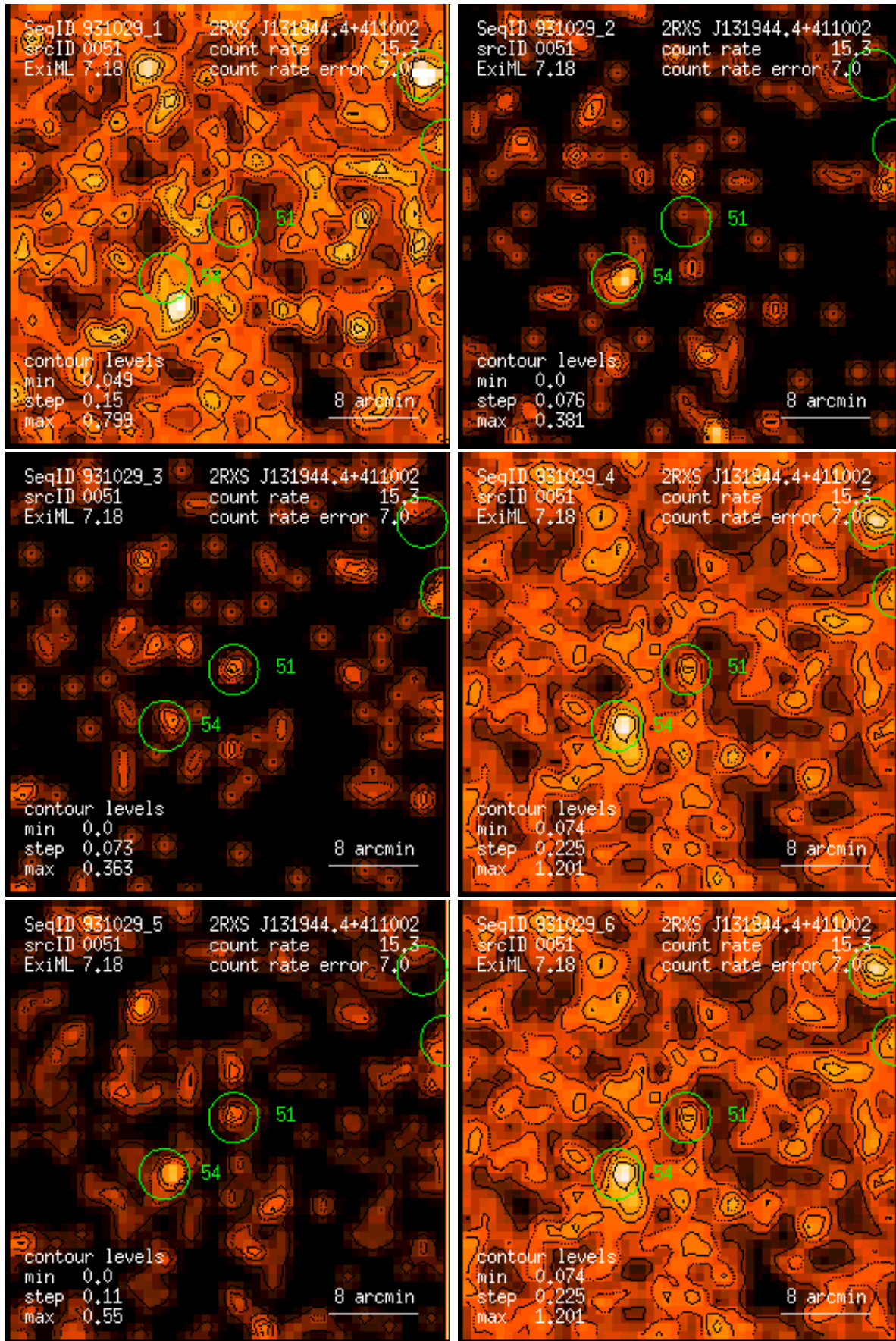
Figure 51: RASS 931029: detection 0051: band rate images, Gaussian filter: (1) PSPC channels 11 – 41, (2) 52 – 90, (3) 91 – 201, (4) 11 – 235, (5) 52 – 201, (6) 11 – 201. Broad band rates in counts/ks. Band rate contour levels in counts/ks/arcmin 2 .
