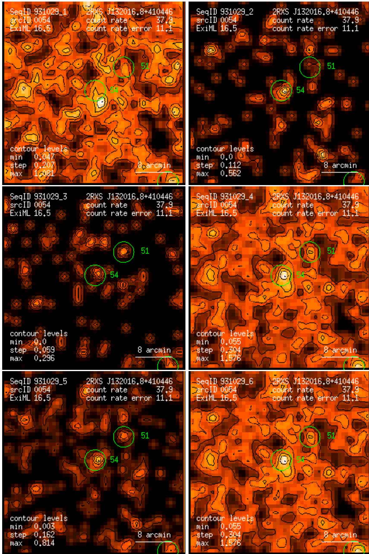
Figure 54: RASS 931029: detection 0054: band rate images, Gaussian filter: (1) PSPC channels 11 – 41, (2) 52 – 90, (3) 91 – 201, (4) 11 – 235, (5) 52 – 201, (6) 11 – 201. Broad band rates in counts/ks. Band rate contour levels in counts/ks/arcmin 2 .
