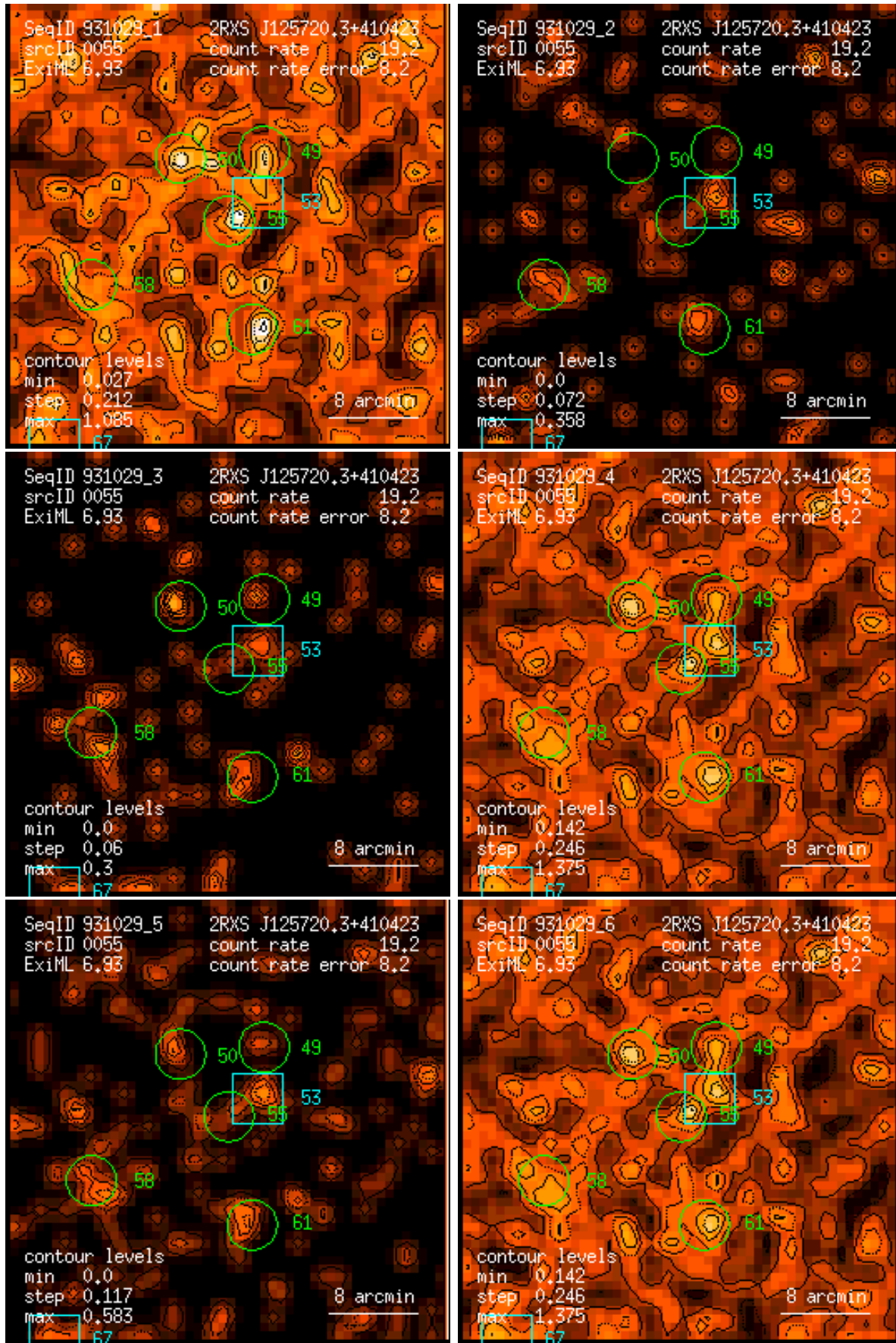
Figure 55: RASS 931029: detection 0055: band rate images, Gaussian filter: (1) PSPC channels 11 – 41, (2) 52 – 90, (3) 91 – 201, (4) 11 – 235, (5) 52 – 201, (6) 11 – 201. Broad band rates in counts/ks. Band rate contour levels in counts/ks/arcmin 2 .
