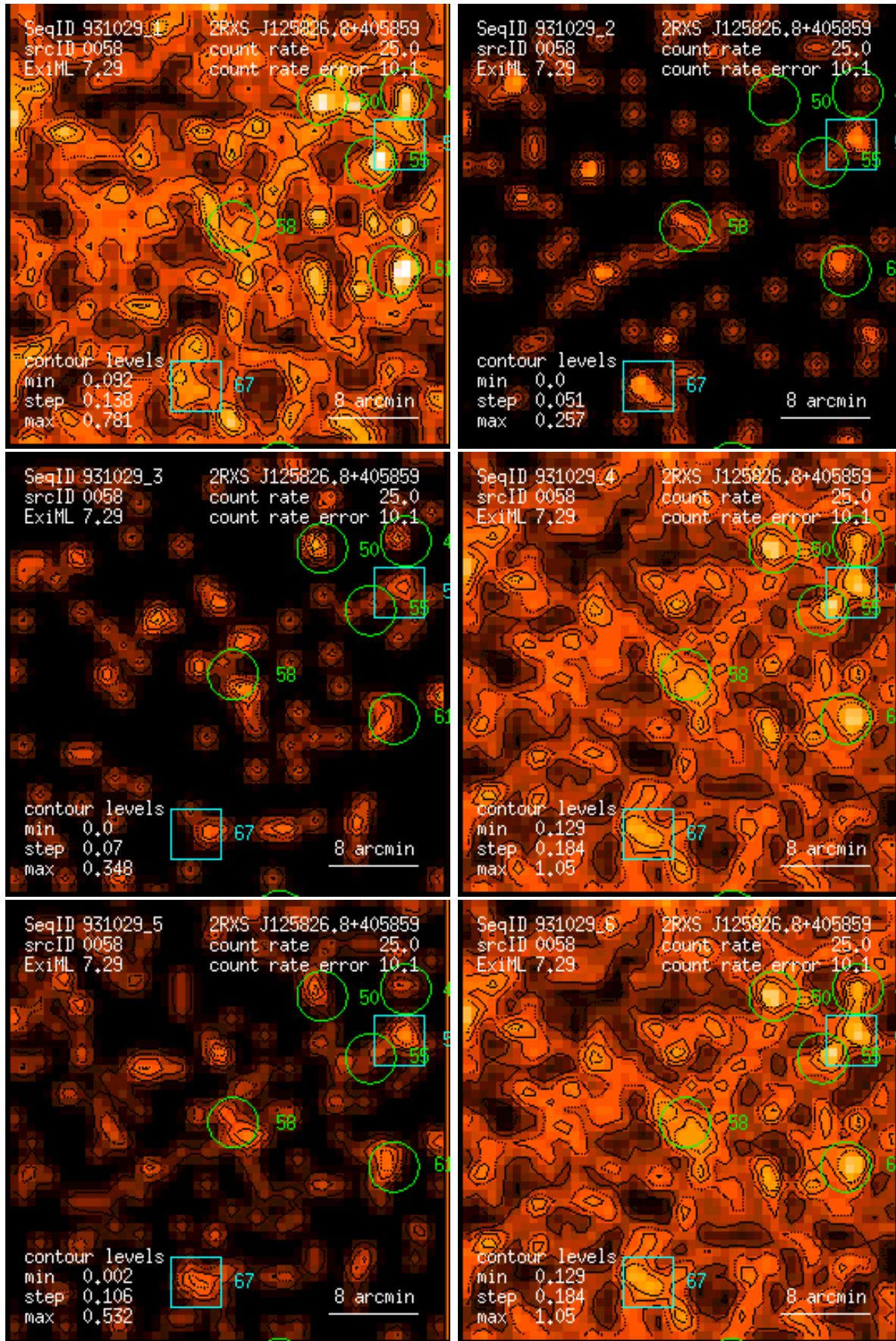
Figure 58: RASS 931029: detection 0058: band rate images, Gaussian filter: (1) PSPC channels 11 – 41, (2) 52 – 90, (3) 91 – 201, (4) 11 – 235, (5) 52 – 201, (6) 11 – 201. Broad band rates in counts/ks. Band rate contour levels in counts/ks/arcmin 2 .
