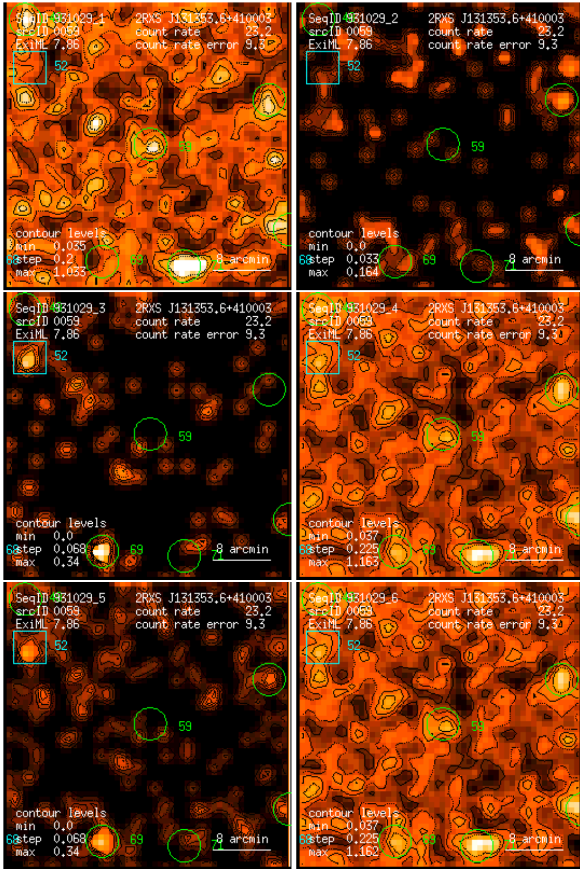
Figure 59: RASS 931029: detection 0059: band rate images, Gaussian filter: (1) PSPC channels 11 – 41, (2) 52 – 90, (3) 91 – 201, (4) 11 – 235, (5) 52 – 201, (6) 11 – 201. Broad band rates in counts/ks. Band rate contour levels in counts/ks/arcmin 2 .
