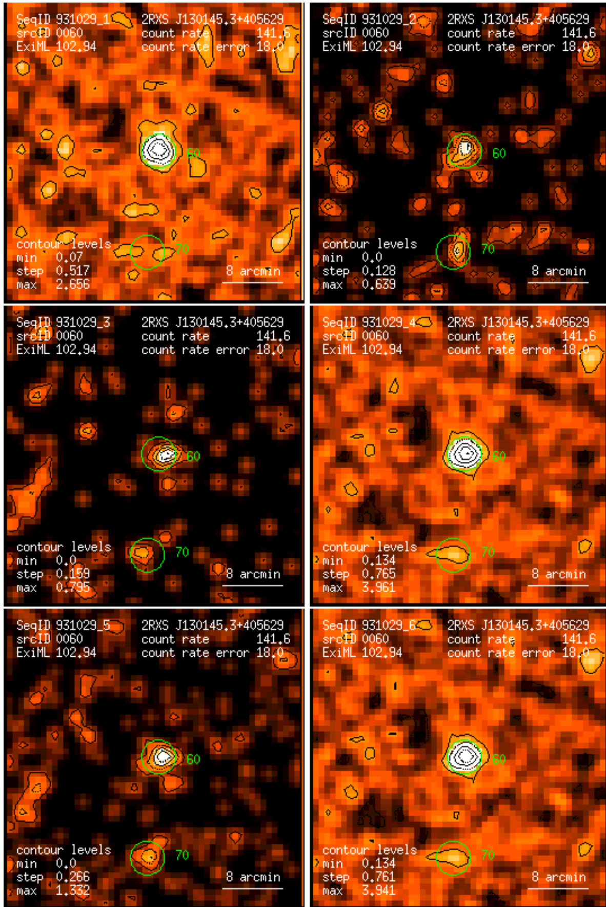
Figure 60: RASS 931029: detection 0060: band rate images, Gaussian filter: (1) PSPC channels 11 – 41, (2) 52 – 90, (3) 91 – 201, (4) 11 – 235, (5) 52 – 201, (6) 11 – 201. Broad band rates in counts/ks. Band rate contour levels in counts/ks/arcmin 2 .
