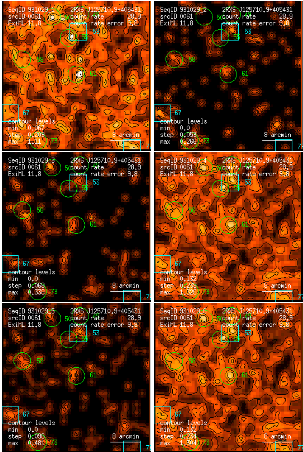
Figure 61: RASS 931029: detection 0061: band rate images, Gaussian filter: (1) PSPC channels 11 – 41, (2) 52 – 90, (3) 91 – 201, (4) 11 – 235, (5) 52 – 201, (6) 11 – 201. Broad band rates in counts/ks. Band rate contour levels in counts/ks/arcmin 2 .
