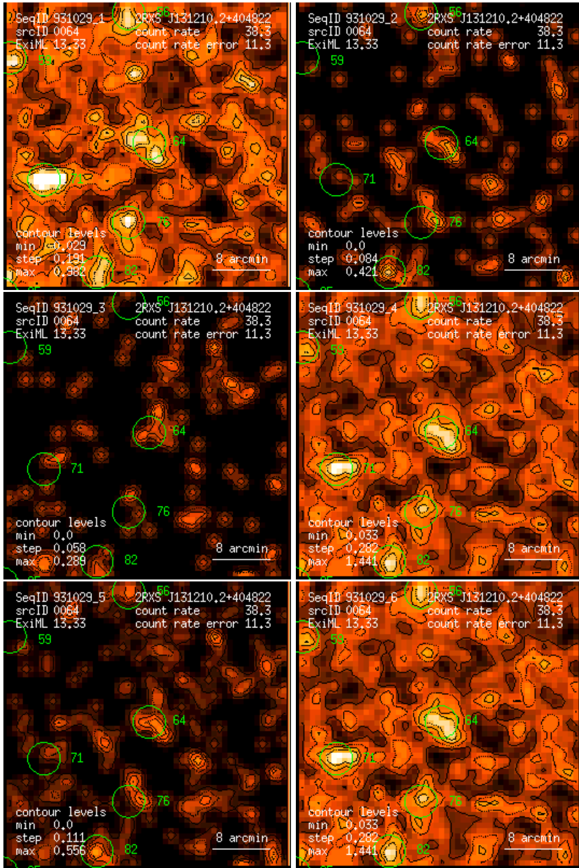
Figure 64: RASS 931029: detection 0064: band rate images, Gaussian filter: (1) PSPC channels 11 – 41, (2) 52 – 90, (3) 91 – 201, (4) 11 – 235, (5) 52 – 201, (6) 11 – 201. Broad band rates in counts/ks. Band rate contour levels in counts/ks/arcmin 2 .
