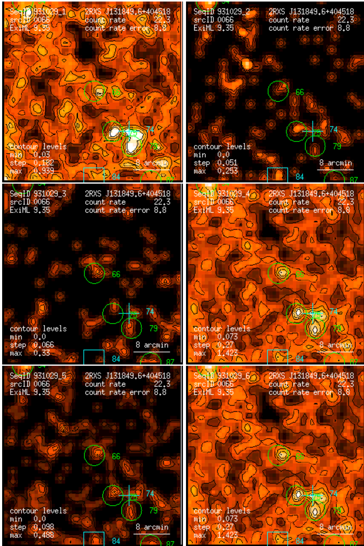
Figure 66: RASS 931029: detection 0066: band rate images, Gaussian filter: (1) PSPC channels 11 – 41, (2) 52 – 90, (3) 91 – 201, (4) 11 – 235, (5) 52 – 201, (6) 11 – 201. Broad band rates in counts/ks. Band rate contour levels in counts/ks/arcmin 2 .
