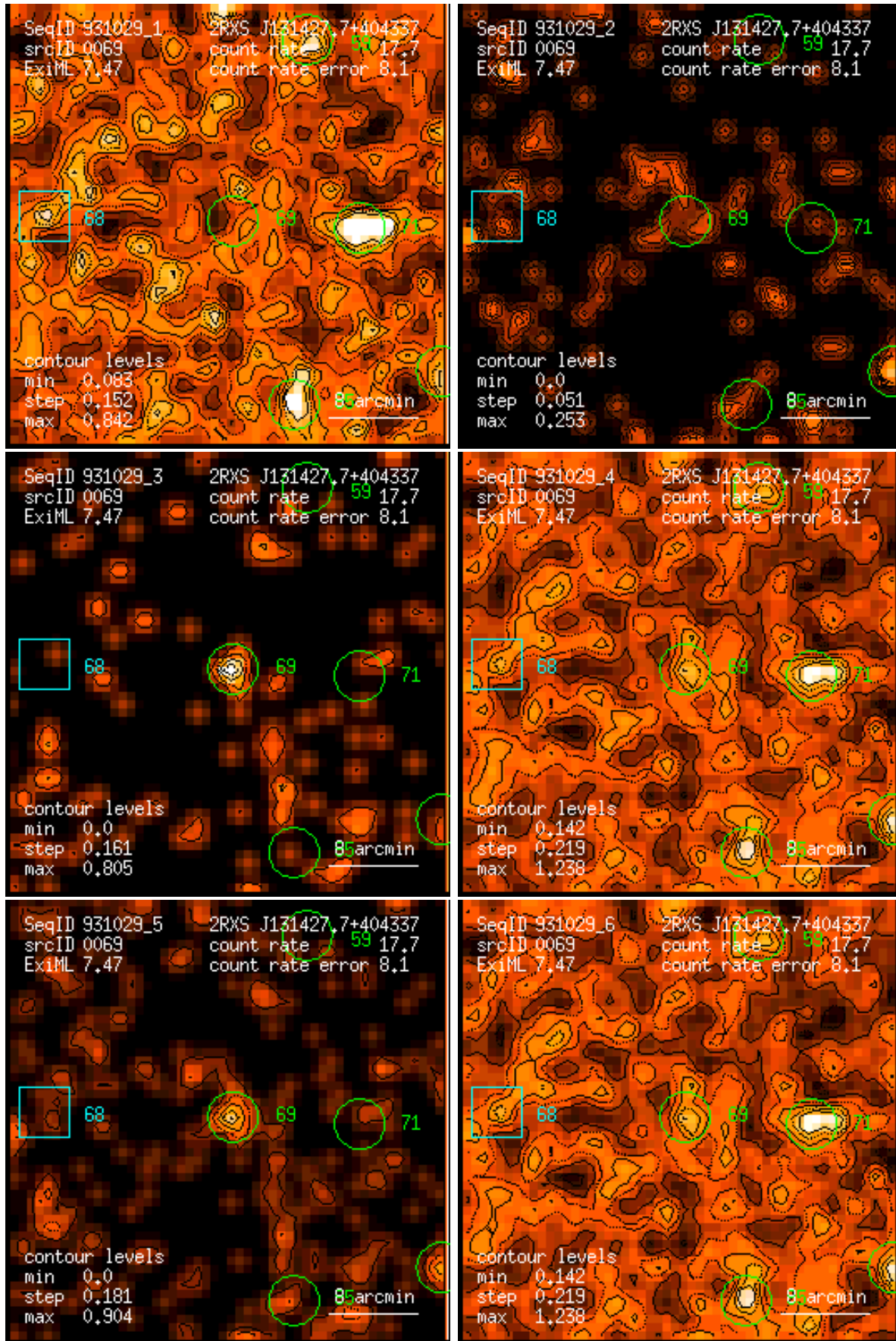
Figure 69: RASS 931029: detection 0069: band rate images, Gaussian filter: (1) PSPC channels 11 – 41, (2) 52 – 90, (3) 91 – 201, (4) 11 – 235, (5) 52 – 201, (6) 11 – 201. Broad band rates in counts/ks. Band rate contour levels in counts/ks/arcmin 2 .
