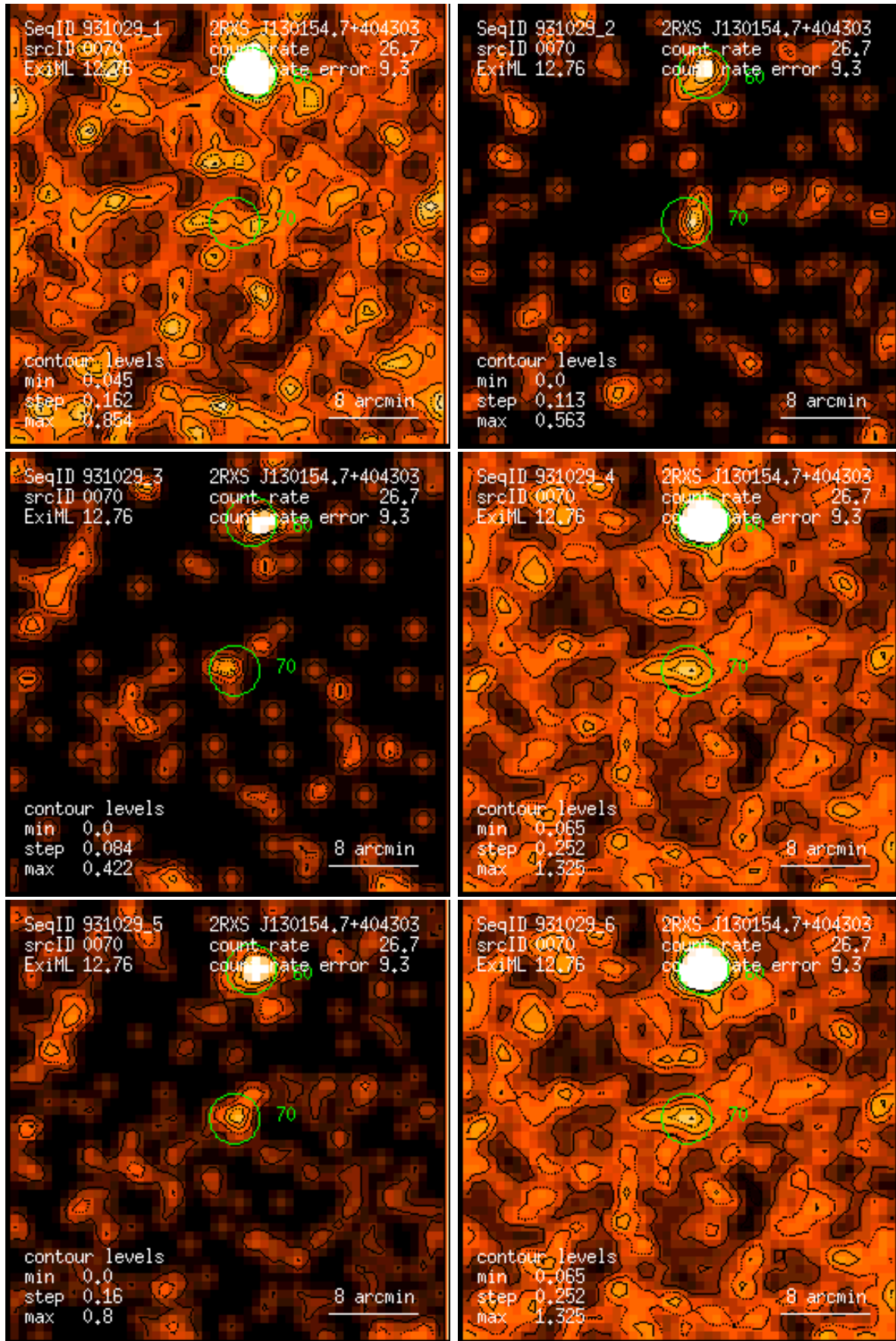
Figure 70: RASS 931029: detection 0070: band rate images, Gaussian filter: (1) PSPC channels 11 – 41, (2) 52 – 90, (3) 91 – 201, (4) 11 – 235, (5) 52 – 201, (6) 11 – 201. Broad band rates in counts/ks. Band rate contour levels in counts/ks/arcmin 2 .
