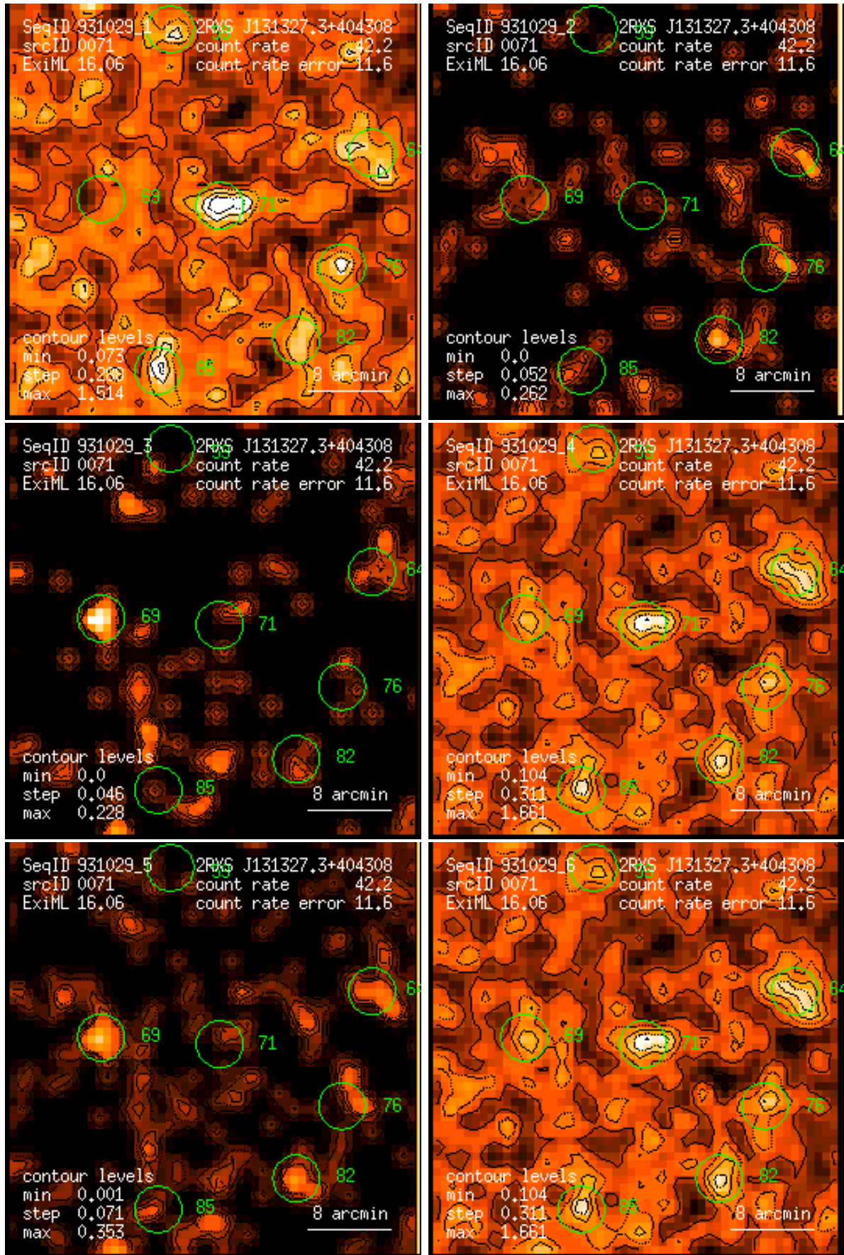
Figure 71: RASS 931029: detection 0071: band rate images, Gaussian filter: (1) PSPC channels 11 – 41, (2) 52 – 90, (3) 91 – 201, (4) 11 – 235, (5) 52 – 201, (6) 11 – 201. Broad band rates in counts/ks. Band rate contour levels in counts/ks/arcmin 2 .
