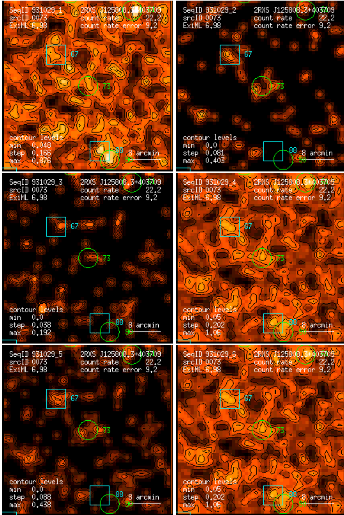
Figure 73: RASS 931029: detection 0073: band rate images, Gaussian filter: (1) PSPC channels 11 – 41, (2) 52 – 90, (3) 91 – 201, (4) 11 – 235, (5) 52 – 201, (6) 11 – 201. Broad band rates in counts/ks. Band rate contour levels in counts/ks/arcmin 2 .
