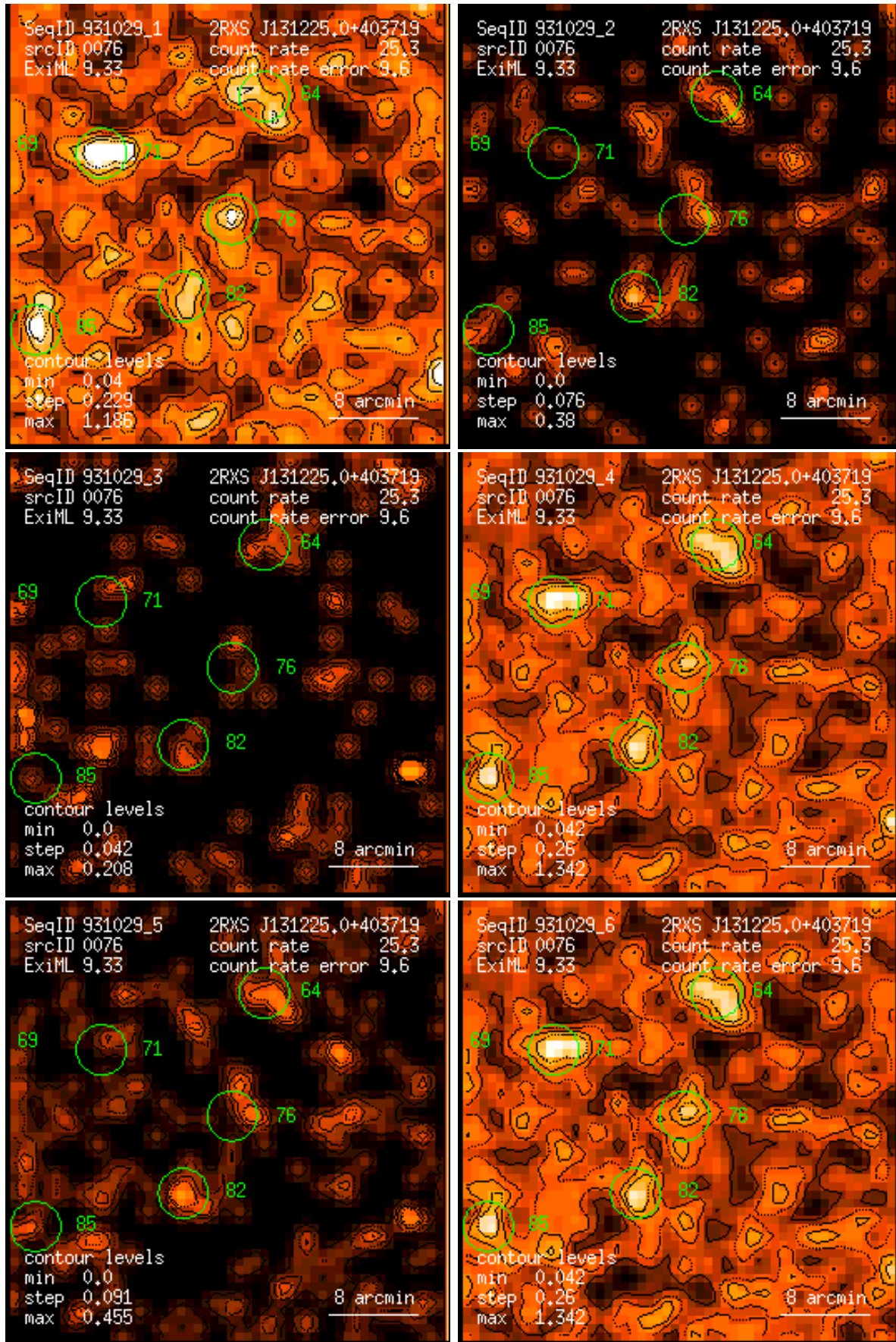
Figure 76: RASS 931029: detection 0076: band rate images, Gaussian filter: (1) PSPC channels 11 – 41, (2) 52 – 90, (3) 91 – 201, (4) 11 – 235, (5) 52 – 201, (6) 11 – 201. Broad band rates in counts/ks. Band rate contour levels in counts/ks/arcmin 2 .
