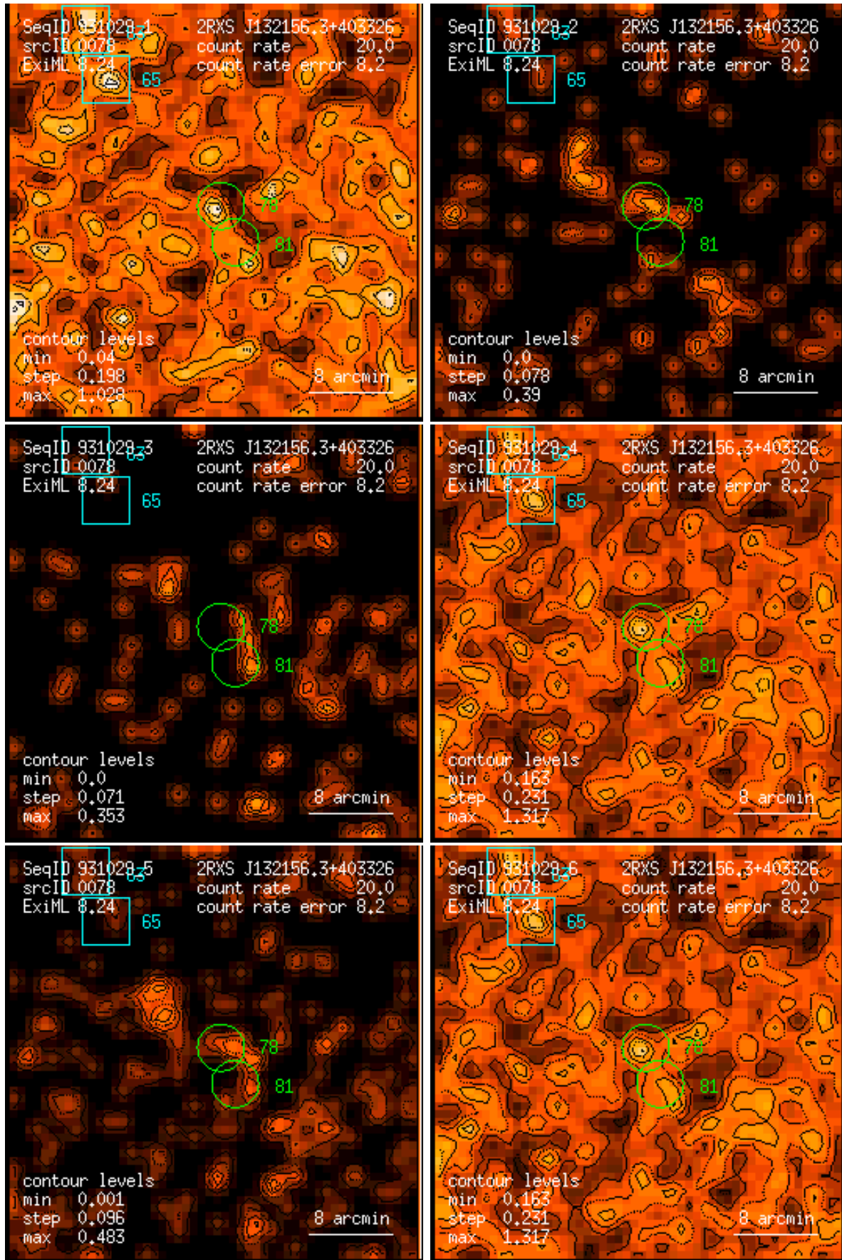
Figure 78: RASS 931029: detection 0078: band rate images, Gaussian filter: (1) PSPC channels 11 – 41, (2) 52 – 90, (3) 91 – 201, (4) 11 – 235, (5) 52 – 201, (6) 11 – 201. Broad band rates in counts/ks. Band rate contour levels in counts/ks/arcmin 2 .
