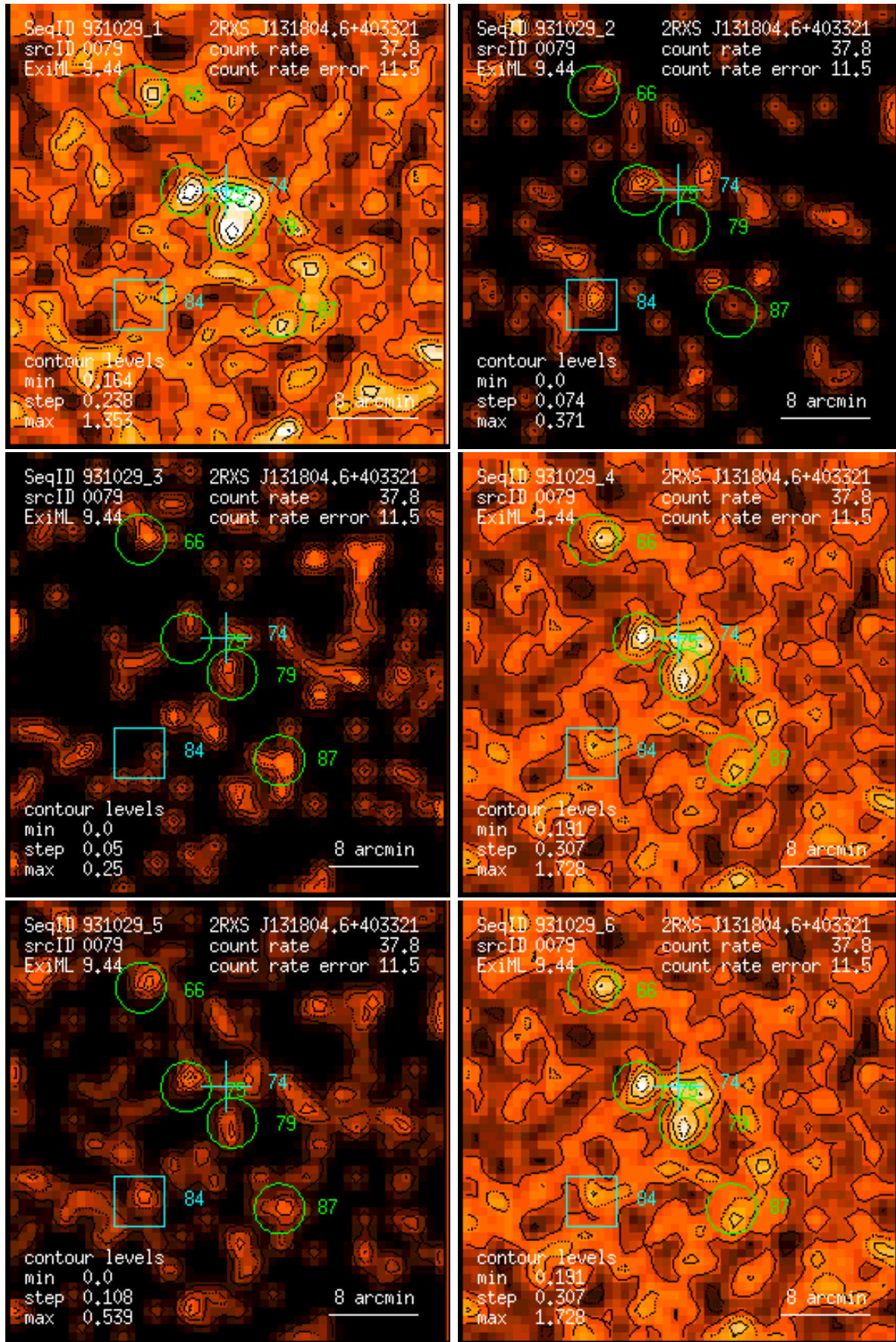
Figure 79: RASS 931029: detection 0079: band rate images, Gaussian filter: (1) PSPC channels 11 – 41, (2) 52 – 90, (3) 91 – 201, (4) 11 – 235, (5) 52 – 201, (6) 11 – 201. Broad band rates in counts/ks. Band rate contour levels in counts/ks/arcmin 2 .
