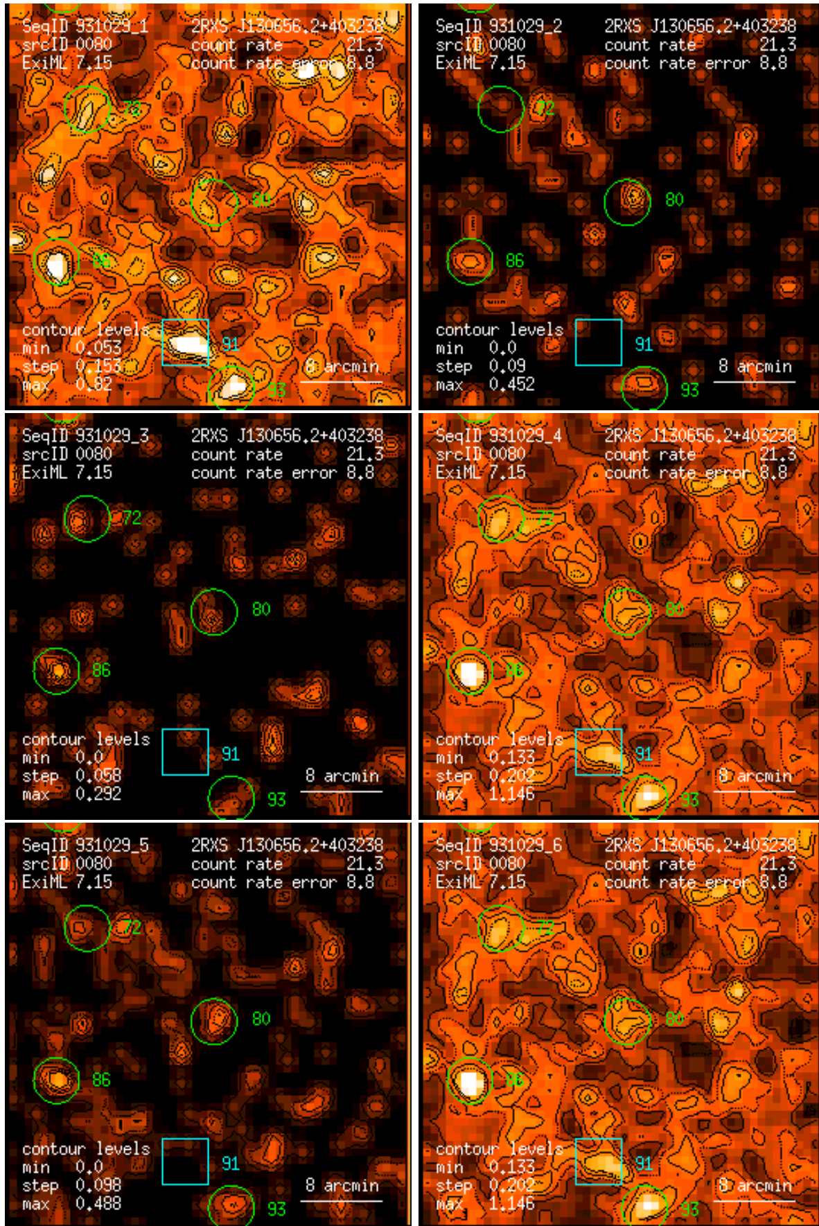
Figure 80: RASS 931029: detection 0080: band rate images, Gaussian filter: (1) PSPC channels 11 – 41, (2) 52 – 90, (3) 91 – 201, (4) 11 – 235, (5) 52 – 201, (6) 11 – 201. Broad band rates in counts/ks. Band rate contour levels in counts/ks/arcmin 2 .
