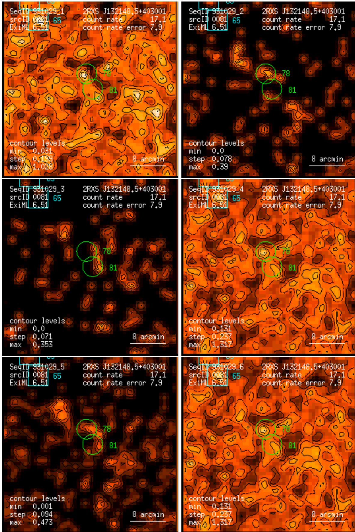
Figure 81: RASS 931029: detection 0081: band rate images, Gaussian filter: (1) PSPC channels 11 – 41, (2) 52 – 90, (3) 91 – 201, (4) 11 – 235, (5) 52 – 201, (6) 11 – 201. Broad band rates in counts/ks. Band rate contour levels in counts/ks/arcmin 2 .
