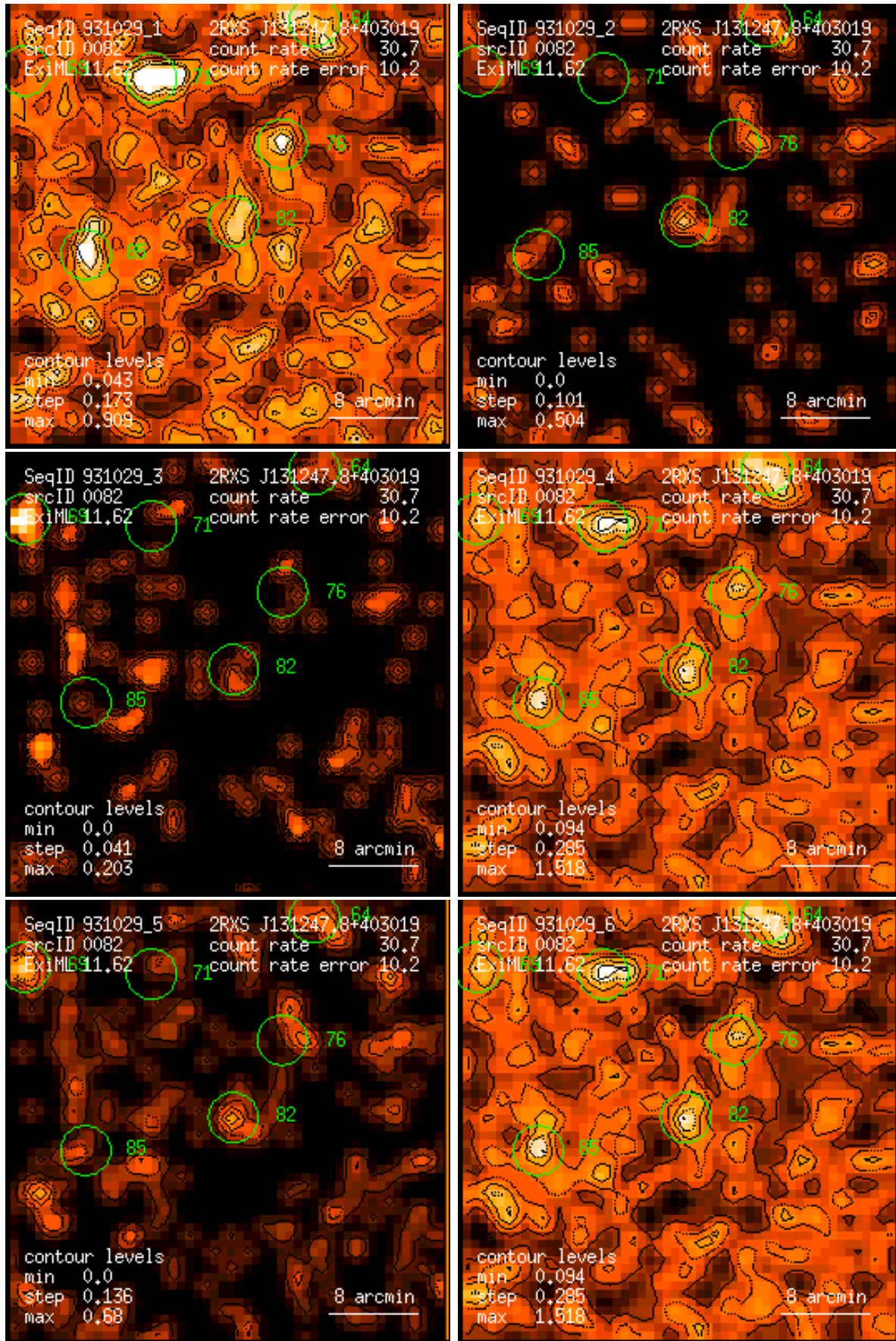
Figure 82: RASS 931029: detection 0082: band rate images, Gaussian filter: (1) PSPC channels 11 – 41, (2) 52 – 90, (3) 91 – 201, (4) 11 – 235, (5) 52 – 201, (6) 11 – 201. Broad band rates in counts/ks. Band rate contour levels in counts/ks/arcmin 2 .
