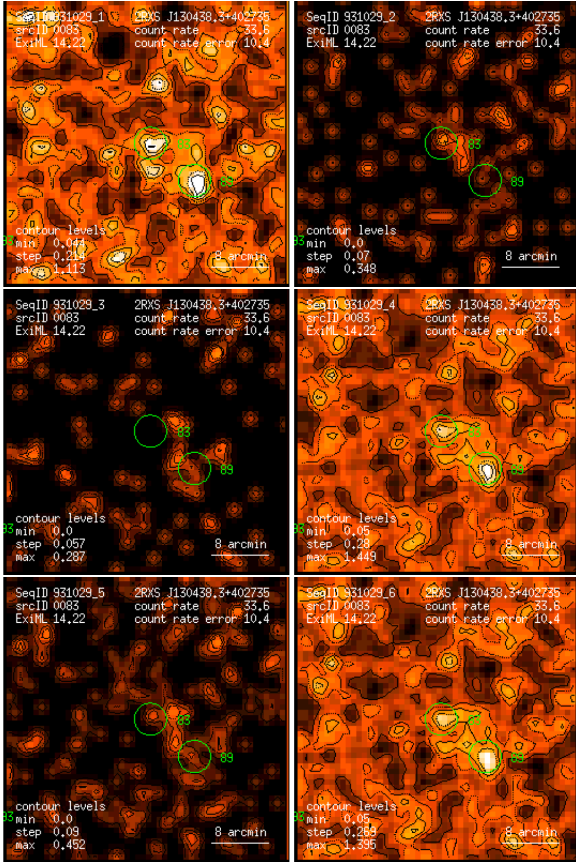
Figure 83: RASS 931029: detection 0083: band rate images, Gaussian filter: (1) PSPC channels 11 – 41, (2) 52 – 90, (3) 91 – 201, (4) 11 – 235, (5) 52 – 201, (6) 11 – 201. Broad band rates in counts/ks. Band rate contour levels in counts/ks/arcmin 2 .
