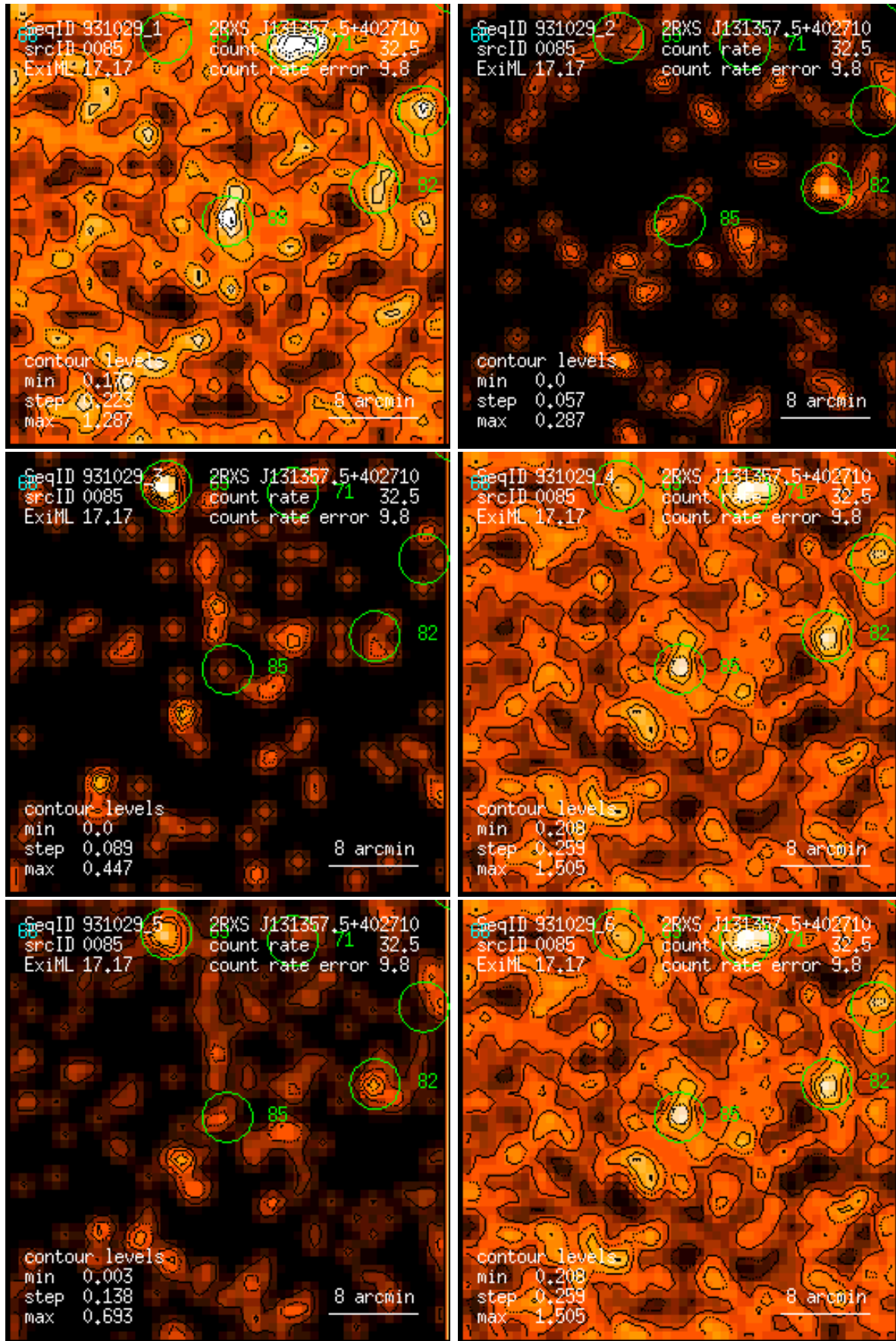
Figure 85: RASS 931029: detection 0085: band rate images, Gaussian filter: (1) PSPC channels 11 – 41, (2) 52 – 90, (3) 91 – 201, (4) 11 – 235, (5) 52 – 201, (6) 11 – 201. Broad band rates in counts/ks. Band rate contour levels in counts/ks/arcmin 2 .
