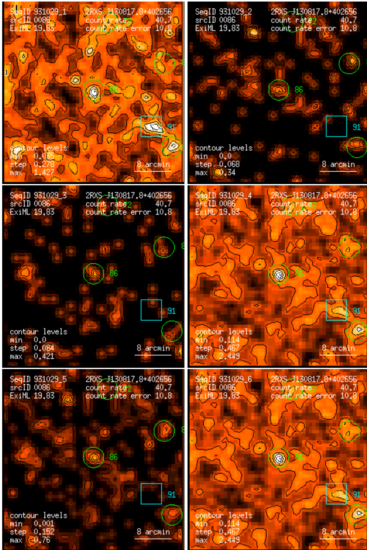
Figure 86: RASS 931029: detection 0086: band rate images, Gaussian filter: (1) PSPC channels 11 – 41, (2) 52 – 90, (3) 91 – 201, (4) 11 – 235, (5) 52 – 201, (6) 11 – 201. Broad band rates in counts/ks. Band rate contour levels in counts/ks/arcmin 2 .
