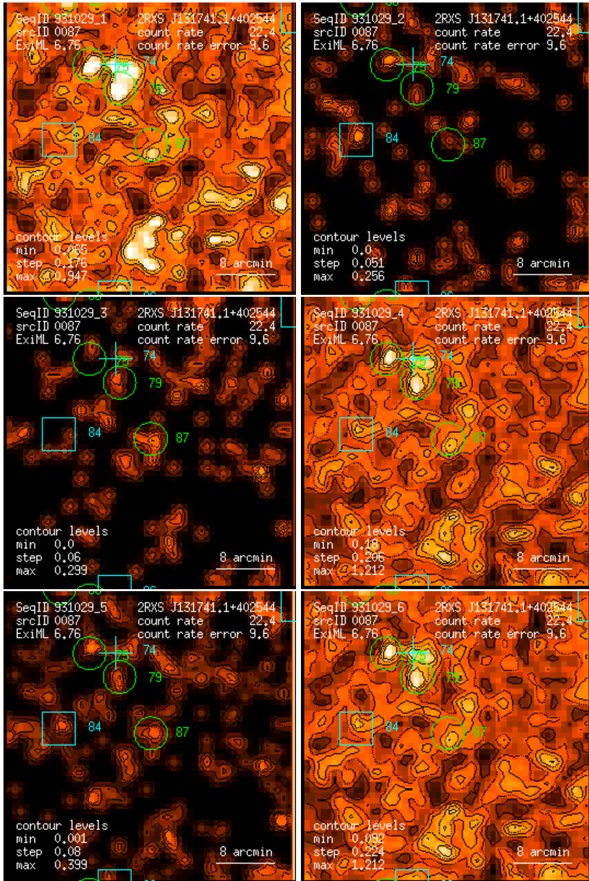
Figure 87: RASS 931029: detection 0087: band rate images, Gaussian filter: (1) PSPC channels 11 – 41, (2) 52 – 90, (3) 91 – 201, (4) 11 – 235, (5) 52 – 201, (6) 11 – 201. Broad band rates in counts/ks. Band rate contour levels in counts/ks/arcmin 2 .
