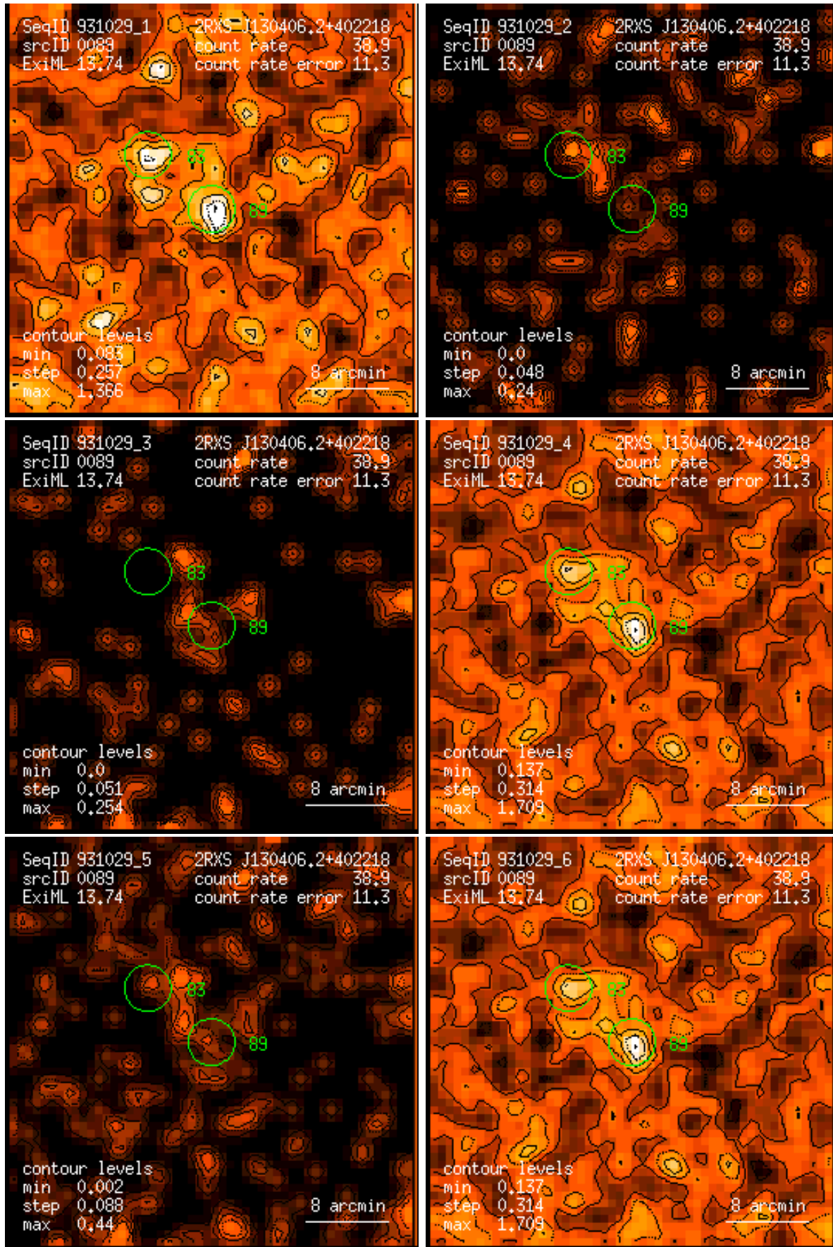
Figure 89: RASS 931029: detection 0089: band rate images, Gaussian filter: (1) PSPC channels 11 – 41, (2) 52 – 90, (3) 91 – 201, (4) 11 – 235, (5) 52 – 201, (6) 11 – 201. Broad band rates in counts/ks. Band rate contour levels in counts/ks/arcmin 2 .
