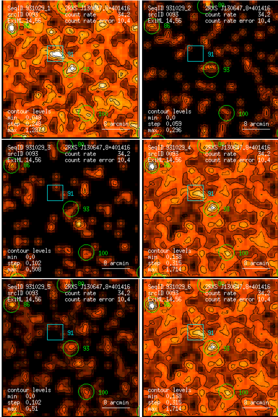
Figure 93: RASS 931029: detection 0093: band rate images, Gaussian filter: (1) PSPC channels 11 – 41, (2) 52 – 90, (3) 91 – 201, (4) 11 – 235, (5) 52 – 201, (6) 11 – 201. Broad band rates in counts/ks. Band rate contour levels in counts/ks/arcmin 2 .
