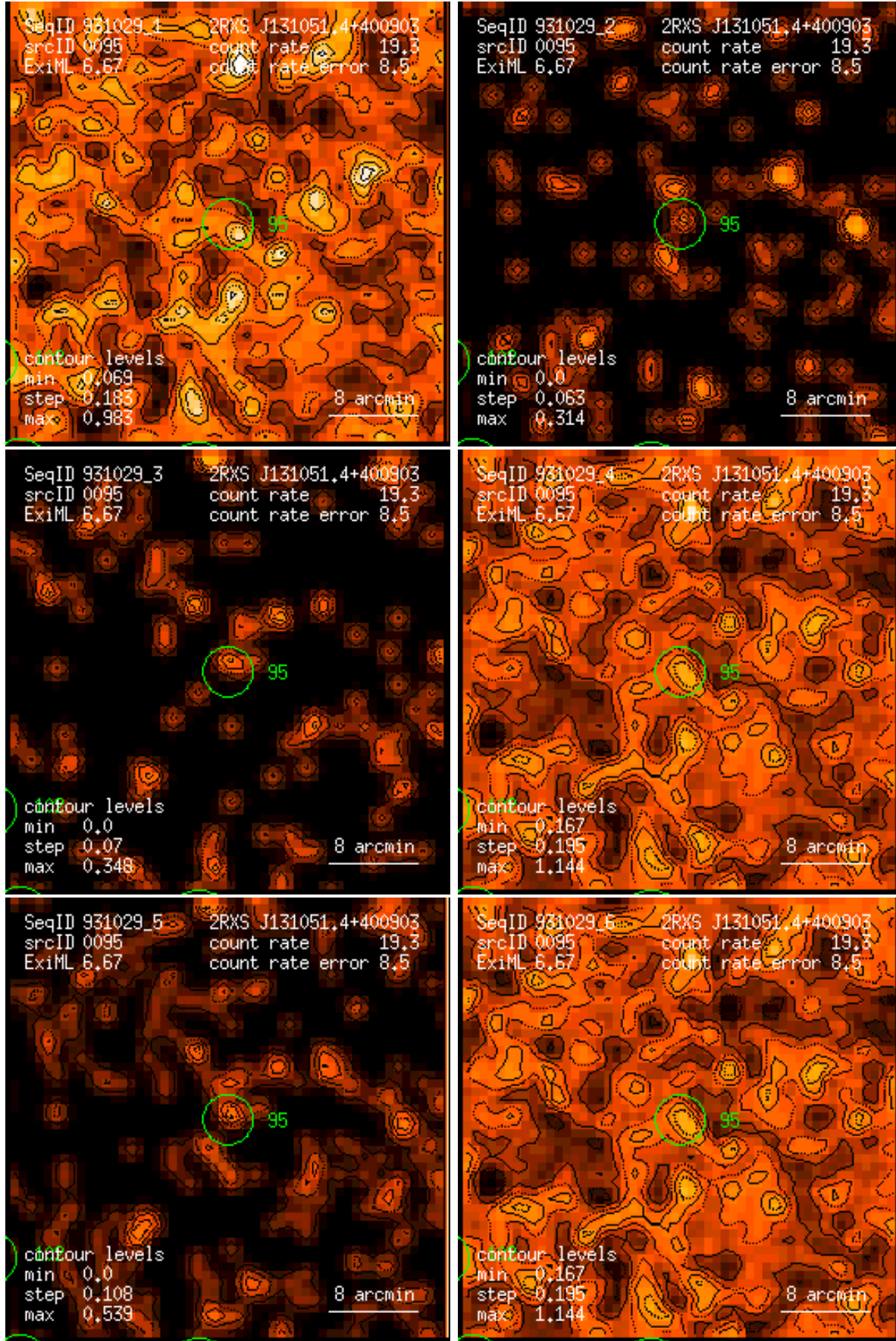
Figure 95: RASS 931029: detection 0095: band rate images, Gaussian filter: (1) PSPC channels 11 – 41, (2) 52 – 90, (3) 91 – 201, (4) 11 – 235, (5) 52 – 201, (6) 11 – 201. Broad band rates in counts/ks. Band rate contour levels in counts/ks/arcmin 2 .
