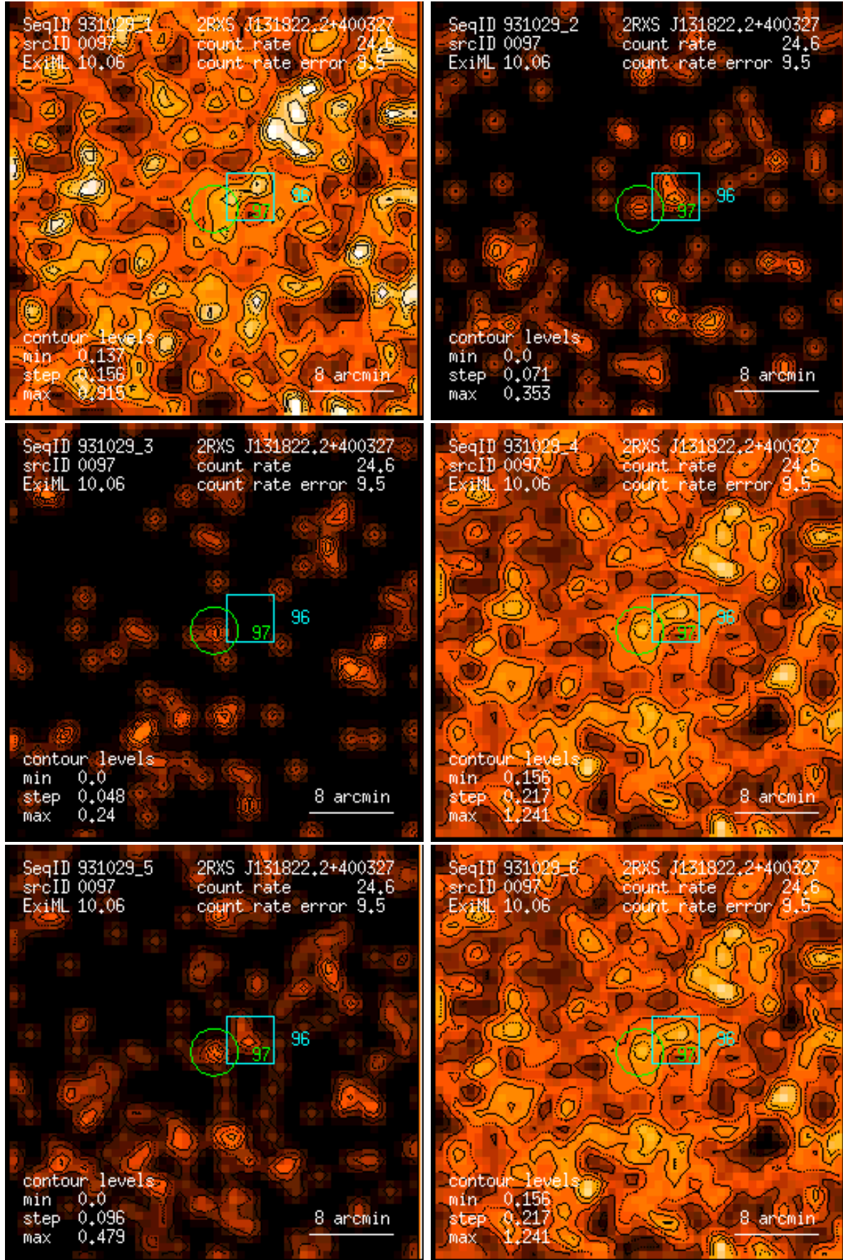
Figure 97: RASS 931029: detection 0097: band rate images, Gaussian filter: (1) PSPC channels 11 – 41, (2) 52 – 90, (3) 91 – 201, (4) 11 – 235, (5) 52 – 201, (6) 11 – 201. Broad band rates in counts/ks. Band rate contour levels in counts/ks/arcmin 2 .
