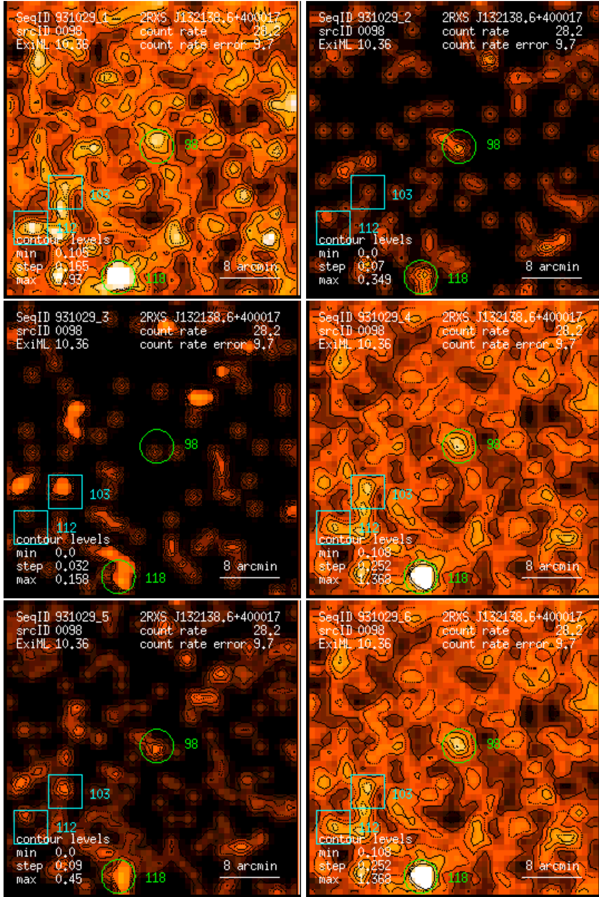
Figure 98: RASS 931029: detection 0098: band rate images, Gaussian filter: (1) PSPC channels 11 – 41, (2) 52 – 90, (3) 91 – 201, (4) 11 – 235, (5) 52 – 201, (6) 11 – 201. Broad band rates in counts/ks. Band rate contour levels in counts/ks/arcmin 2 .
