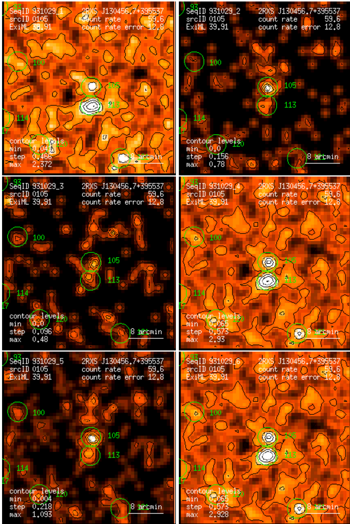
Figure 105: RASS 931029: detection 0105: band rate images, Gaussian filter: (1) PSPC channels 11 – 41, (2) 52 – 90, (3) 91 – 201, (4) 11 – 235, (5) 52 – 201, (6) 11 – 201. Broad band rates in counts/ks. Band rate contour levels in counts/ks/arcmin 2 .
