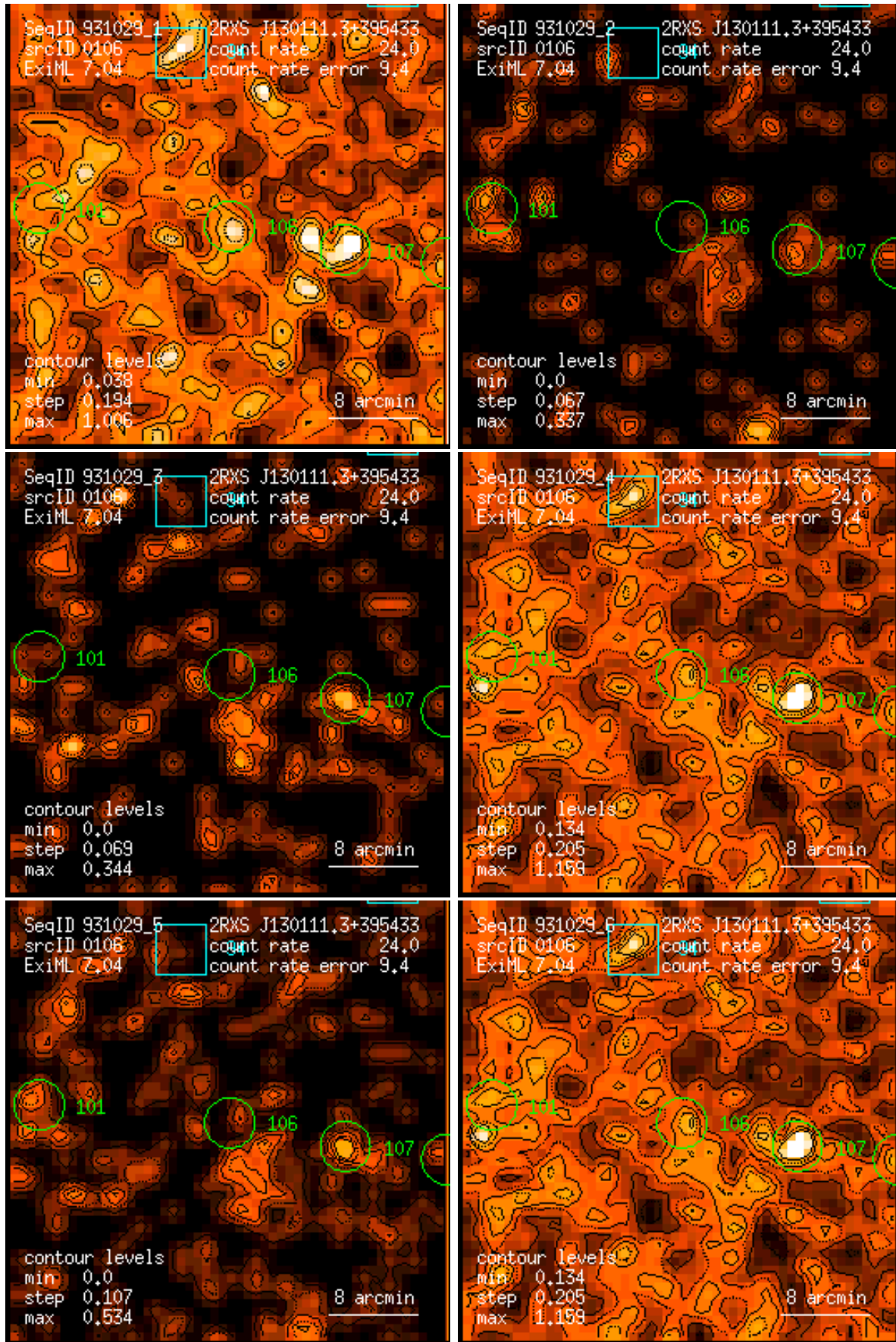
Figure 106: RASS 931029: detection 0106: band rate images, Gaussian filter: (1) PSPC channels 11 – 41, (2) 52 – 90, (3) 91 – 201, (4) 11 – 235, (5) 52 – 201, (6) 11 – 201. Broad band rates in counts/ks. Band rate contour levels in counts/ks/arcmin 2 .
