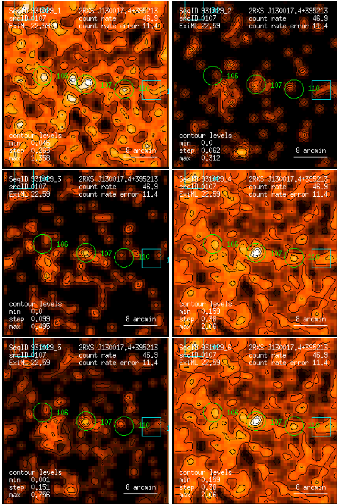
Figure 107: RASS 931029: detection 0107: band rate images, Gaussian filter: (1) PSPC channels 11 – 41, (2) 52 – 90, (3) 91 – 201, (4) 11 – 235, (5) 52 – 201, (6) 11 – 201. Broad band rates in counts/ks. Band rate contour levels in counts/ks/arcmin 2 .
