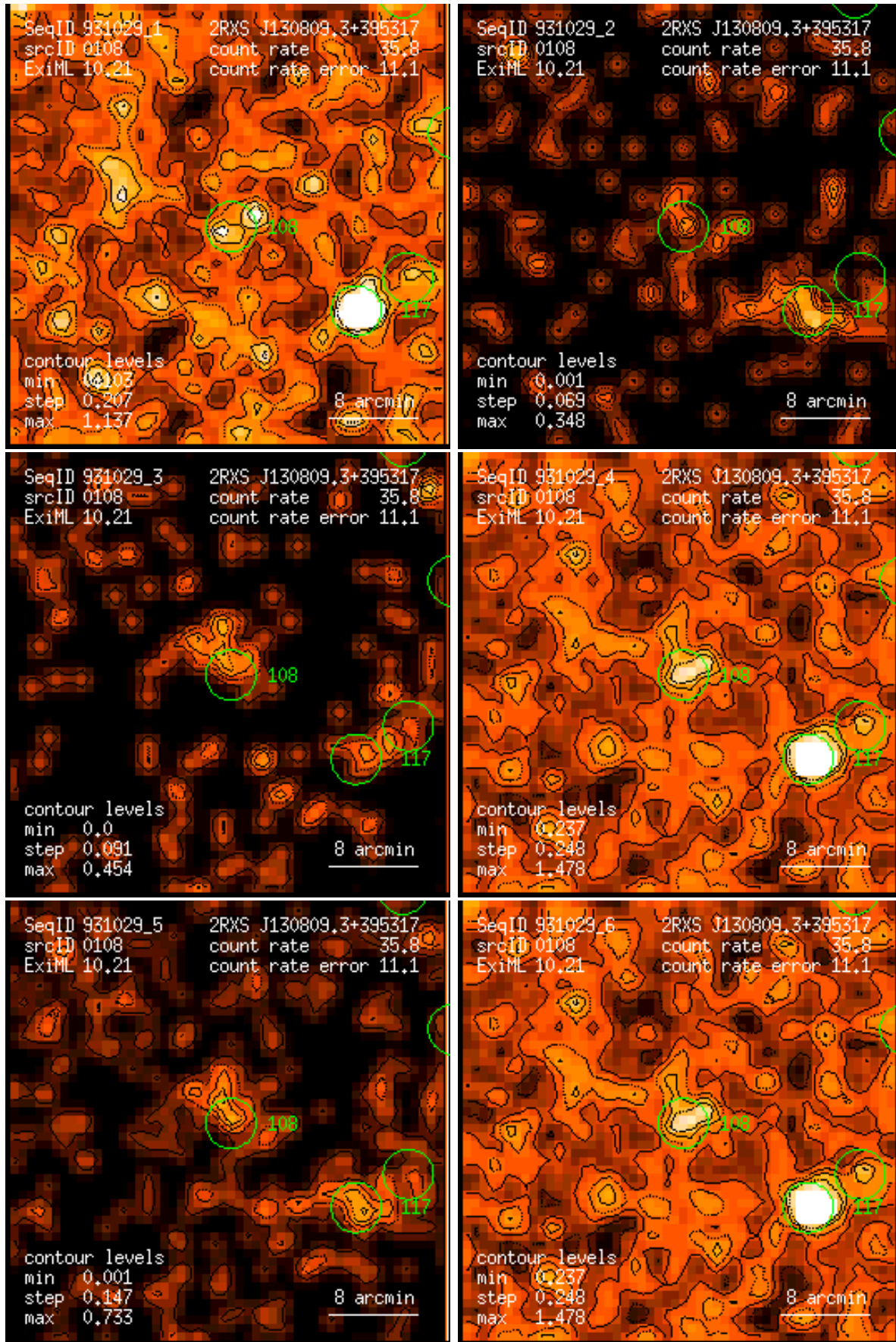
Figure 108: RASS 931029: detection 0108: band rate images, Gaussian filter: (1) PSPC channels 11 – 41, (2) 52 – 90, (3) 91 – 201, (4) 11 – 235, (5) 52 – 201, (6) 11 – 201. Broad band rates in counts/ks. Band rate contour levels in counts/ks/arcmin 2 .
