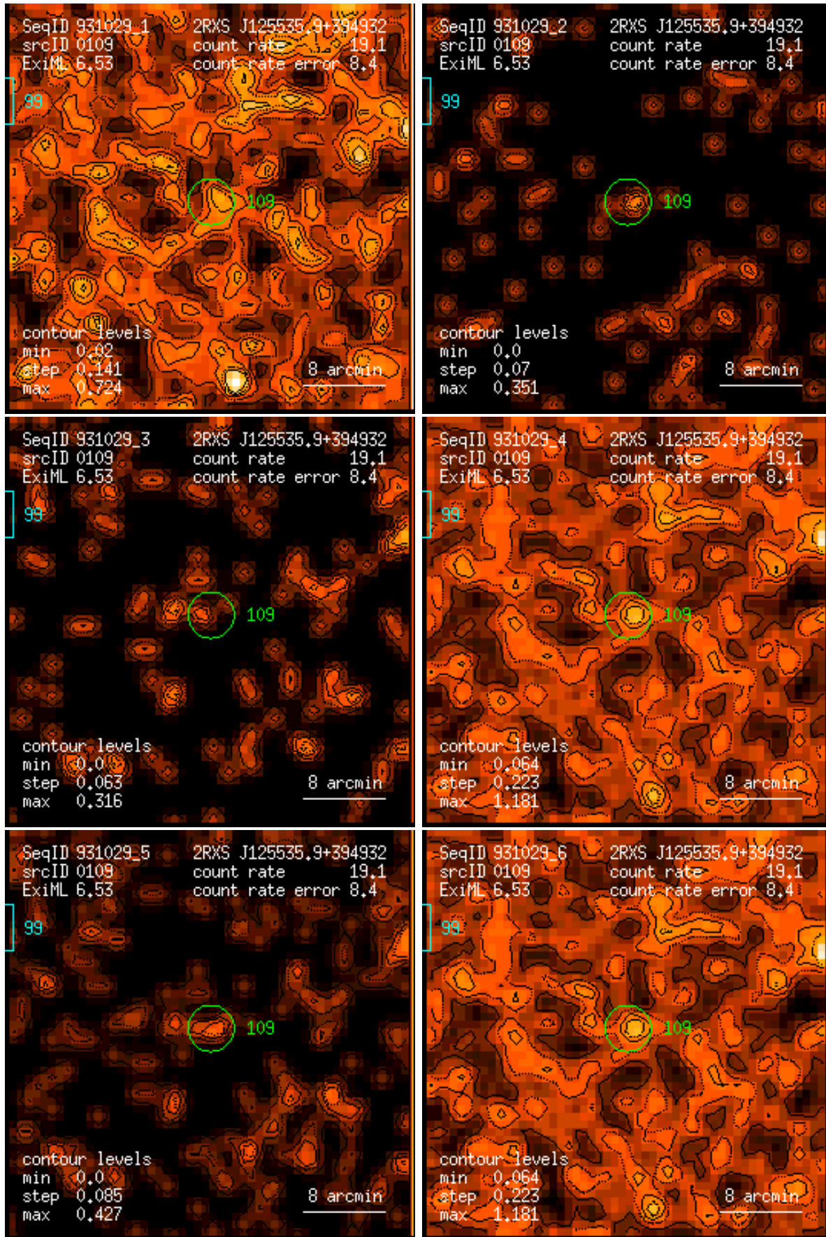
Figure 109: RASS 931029: detection 0109: band rate images, Gaussian filter: (1) PSPC channels 11 – 41, (2) 52 – 90, (3) 91 – 201, (4) 11 – 235, (5) 52 – 201, (6) 11 – 201. Broad band rates in counts/ks. Band rate contour levels in counts/ks/arcmin 2 .
