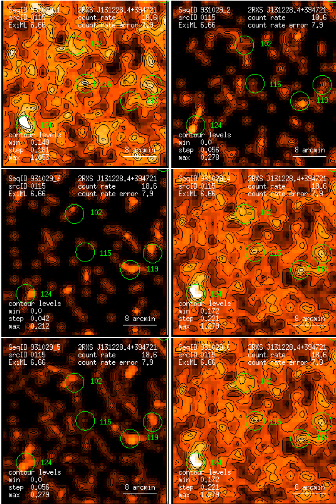
Figure 115: RASS 931029: detection 0115: band rate images, Gaussian filter: (1) PSPC channels 11 – 41, (2) 52 – 90, (3) 91 – 201, (4) 11 – 235, (5) 52 – 201, (6) 11 – 201. Broad band rates in counts/ks. Band rate contour levels in counts/ks/arcmin 2 .
