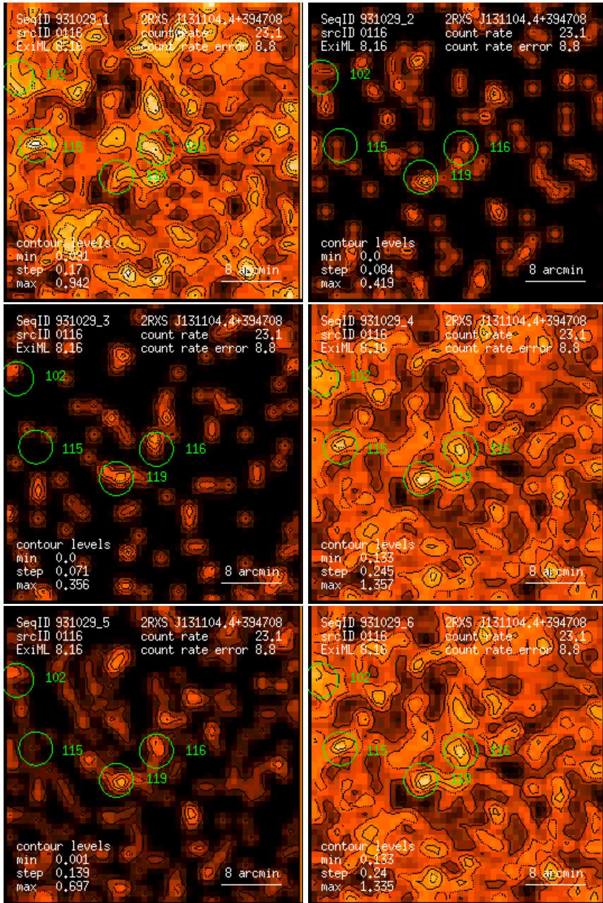
Figure 116: RASS 931029: detection 0116: band rate images, Gaussian filter: (1) PSPC channels 11 – 41, (2) 52 – 90, (3) 91 – 201, (4) 11 – 235, (5) 52 – 201, (6) 11 – 201. Broad band rates in counts/ks. Band rate contour levels in counts/ks/arcmin 2 .
