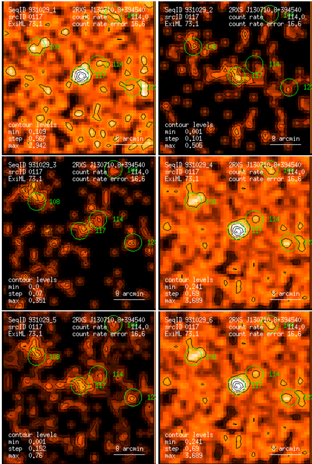
Figure 117: RASS 931029: detection 0117: band rate images, Gaussian filter: (1) PSPPC channels 11 – 41, (2) 52 – 90, (3) 91 – 201, (4) 11 – 235, (5) 52 – 201, (6) 11 – 201. Broad band rates in counts/ks. Band rate contour levels in counts/ks/arcmin 2 .
