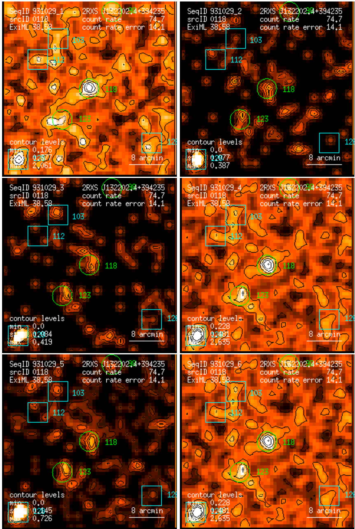
Figure 118: RASS 931029: detection 0118: band rate images, Gaussian filter: (1) PSPC channels 11 – 41, (2) 52 – 90, (3) 91 – 201, (4) 11 – 235, (5) 52 – 201, (6) 11 – 201. Broad band rates in counts/ks. Band rate contour levels in counts/ks/arcmin 2 .
