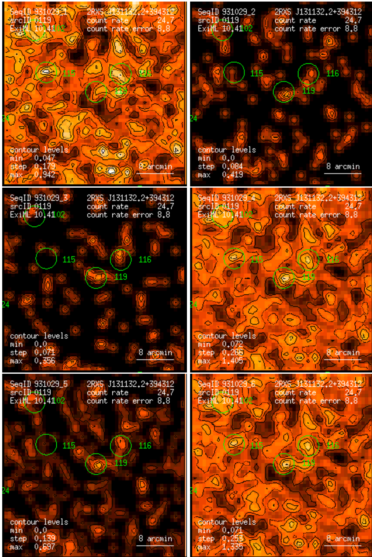
Figure 119: RASS 931029: detection 0119: band rate images, Gaussian filter: (1) PSPC channels 11 – 41, (2) 52 – 90, (3) 91 – 201, (4) 11 – 235, (5) 52 – 201, (6) 11 – 201. Broad band rates in counts/ks. Band rate contour levels in counts/ks/arcmin 2 .
