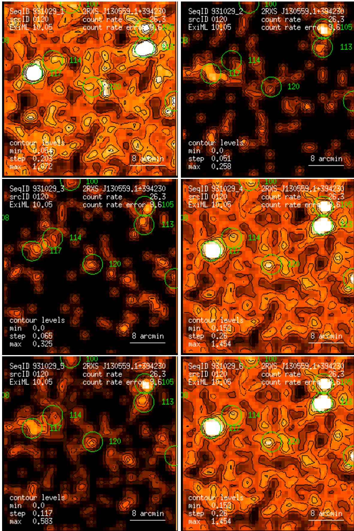
Figure 120: RASS 931029: detection 0120: band rate images, Gaussian filter: (1) PSPC channels 11 – 41, (2) 52 – 90, (3) 91 – 201, (4) 11 – 235, (5) 52 – 201, (6) 11 – 201. Broad band rates in counts/ks. Band rate contour levels in counts/ks/arcmin 2 .
