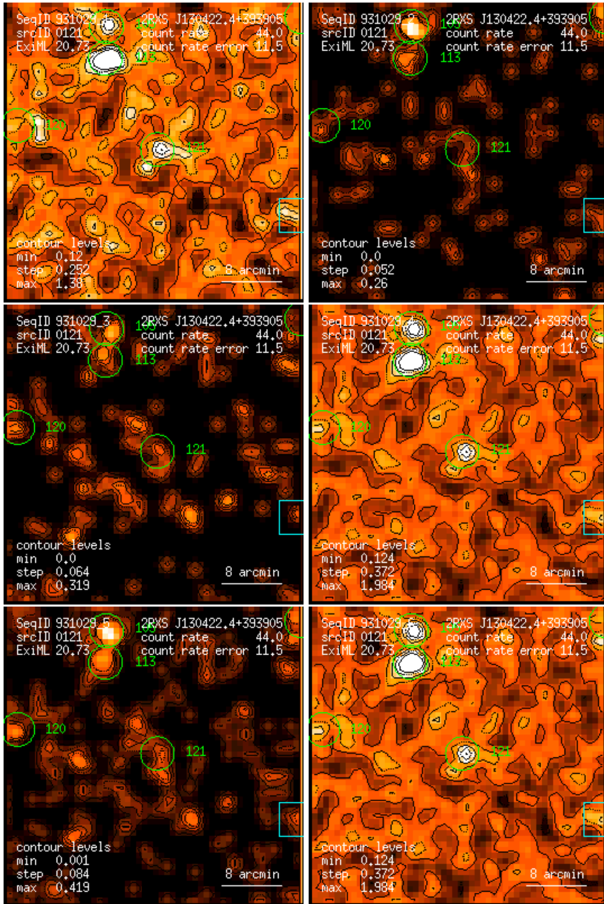
Figure 121: RASS 931029: detection 0121: band rate images, Gaussian filter: (1) PSPC channels 11 – 41, (2) 52 – 90, (3) 91 – 201, (4) 11 – 235, (5) 52 – 201, (6) 11 – 201. Broad band rates in counts/ks. Band rate contour levels in counts/ks/arcmin 2 .
