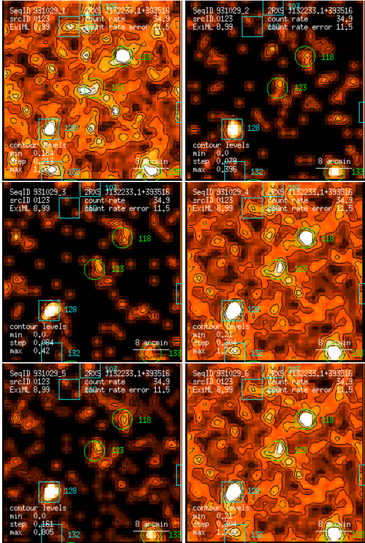
Figure 123: RASS 931029: detection 0123: band rate images, Gaussian filter: (1) PSPC channels 11 – 41, (2) 52 – 90, (3) 91 – 201, (4) 11 – 235, (5) 52 – 201, (6) 11 – 201. Broad band rates in counts/ks. Band rate contour levels in counts/ks/arcmin 2 .
