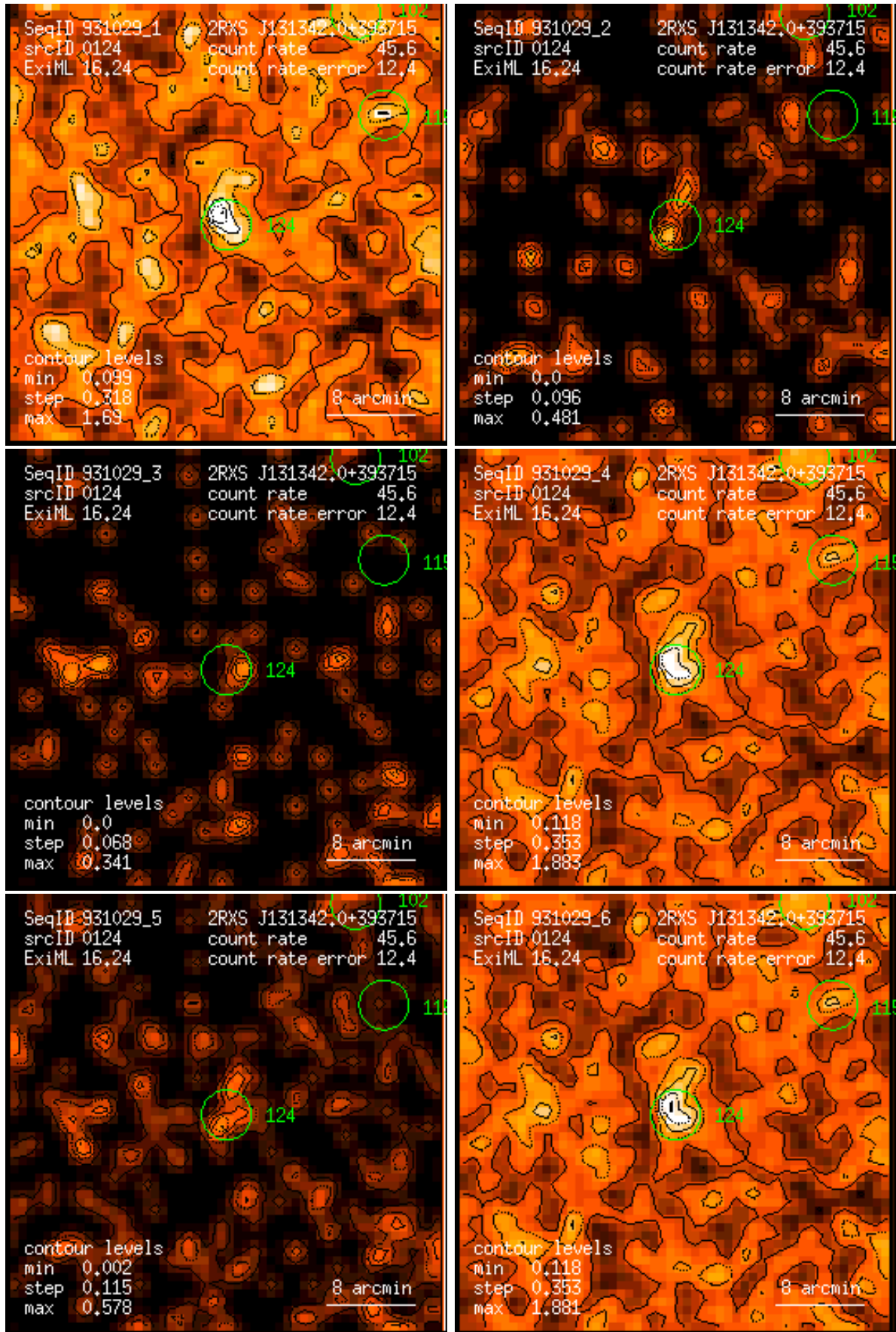
Figure 124: RASS 931029: detection 0124: band rate images, Gaussian filter: (1) PSPC channels 11 – 41, (2) 52 – 90, (3) 91 – 201, (4) 11 – 235, (5) 52 – 201, (6) 11 – 201. Broad band rates in counts/ks. Band rate contour levels in counts/ks/arcmin 2 .
