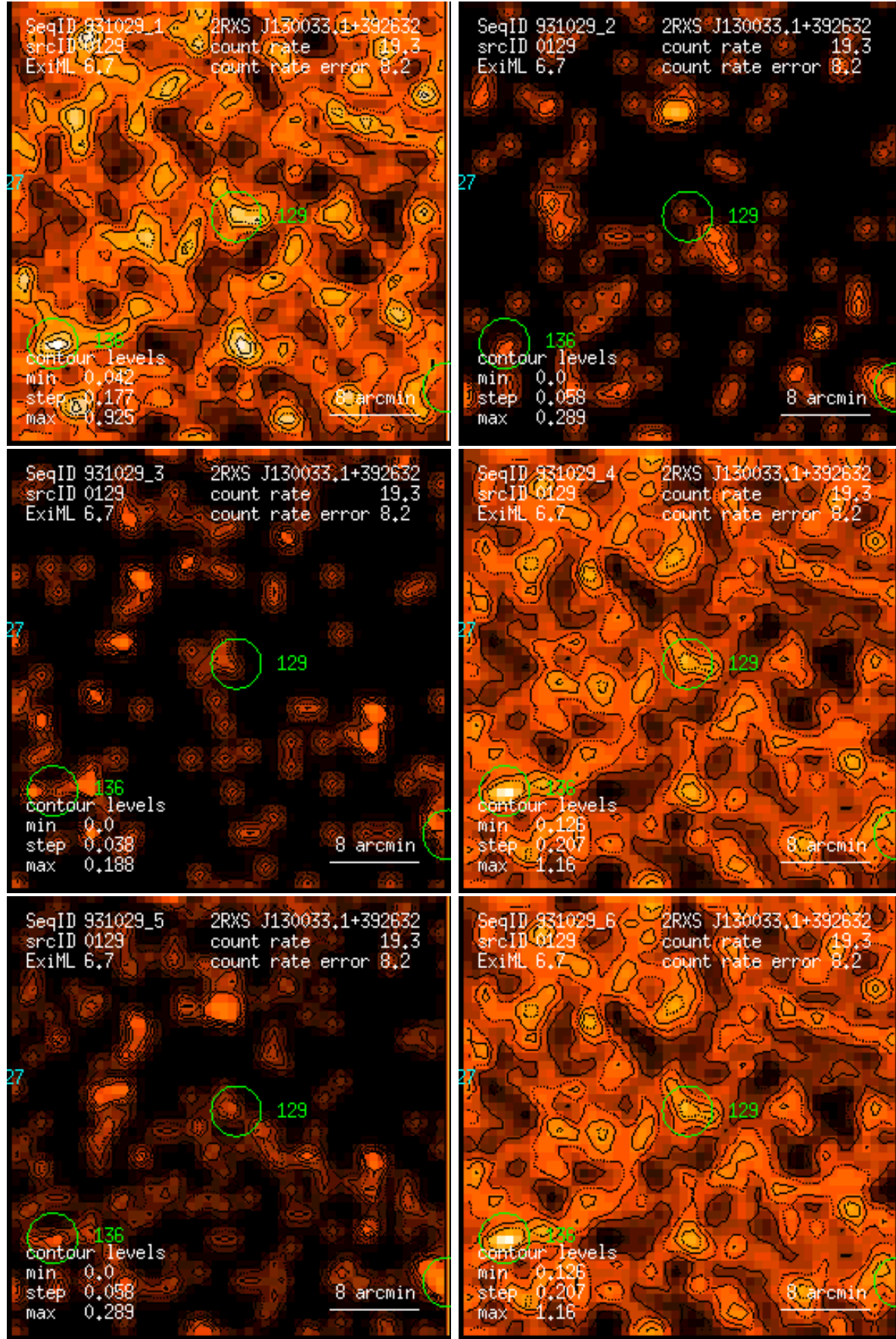
Figure 129: RASS 931029: detection 0129: band rate images, Gaussian filter: (1) PSPC channels 11 – 41, (2) 52 – 90, (3) 91 – 201, (4) 11 – 235, (5) 52 – 201, (6) 11 – 201. Broad band rates in counts/ks. Band rate contour levels in counts/ks/arcmin 2 .
