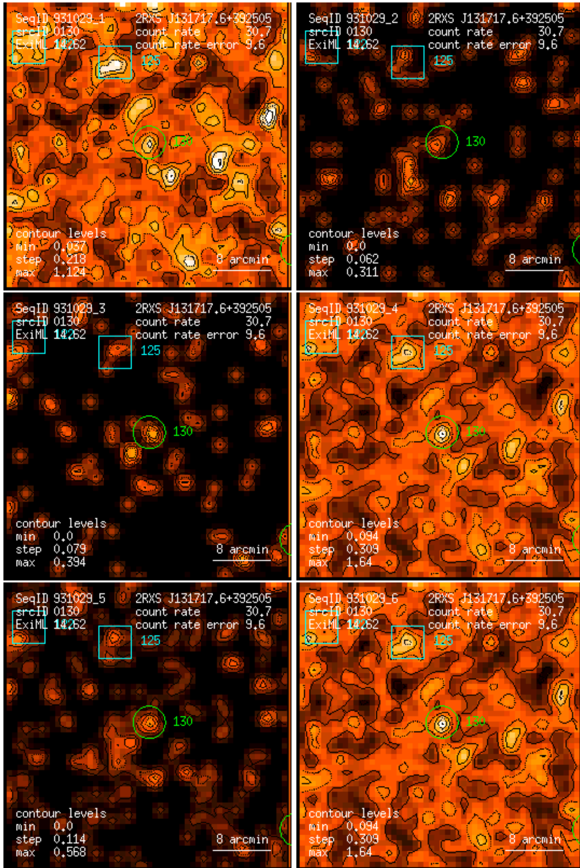
Figure 130: RASS 931029: detection 0130: band rate images, Gaussian filter: (1) PSPC channels 11 – 41, (2) 52 – 90, (3) 91 – 201, (4) 11 – 235, (5) 52 – 201, (6) 11 – 201. Broad band rates in counts/ks. Band rate contour levels in counts/ks/arcmin 2 .
